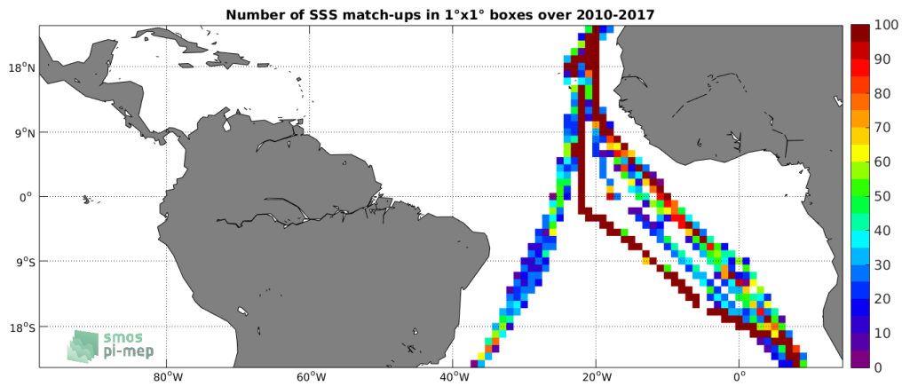
Figure 4: Number of SSS match-ups between TSG-POLARSTERN SSS and the SMOS L3 v2 - Monthly - 0.25 Deg (CATDS-CECOS-IFREMER) SSS product for the Tropical Atlantic Ocean Pi-MEP region over 1^\circ \times 1^\circ boxes and for the full satellite product period.
