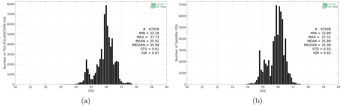
Figure 2: Histograms of SSS from TSG-POLARSTERN (a) and SMOS L3 v2 - Monthly - 0.25 Deg (CATDS-CECOS-IFREMER) (b) considering all match-up pairs per bins of 0.1 over the Tropical Atlantic Ocean Pi-MEP region and for the full satellite product period.
