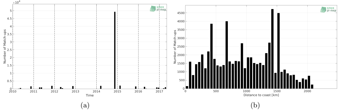
Figure 1: Number of match-ups between TSG-POLARSTERN and SMOS L3 v2 - Monthly - 0.25 Deg (CATDS-CECOS-IFREMER) SSS as a function of time (a) and as function of the distance to coast (b) over the Tropical Atlantic Ocean Pi-MEP region and for the full satellite product period.
