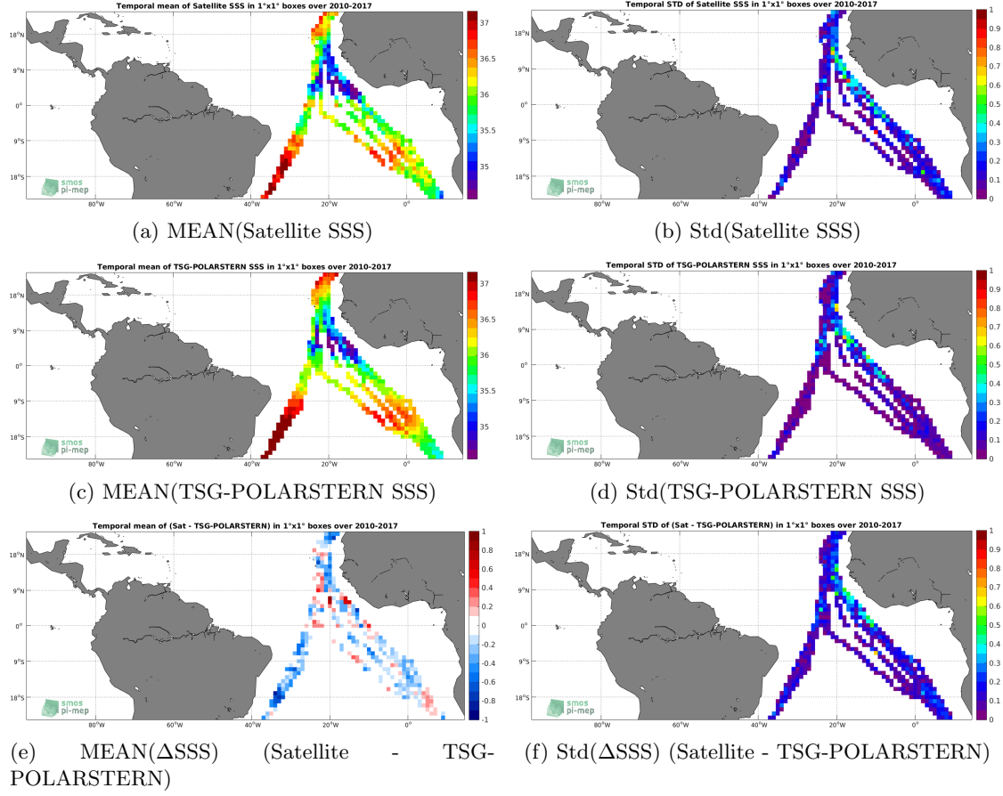
Figure 6: Temporal mean (left) and Std (right) of SSS from SMOS L3 v2 - Monthly - 0.25 Deg (CATDS-CECOS-IFREMER) (top), TSG-POLARSTERN (middle), and of \Delta SSS (Satellite - TSG-POLARSTERN). Only match-up pairs are used to generate these maps.
