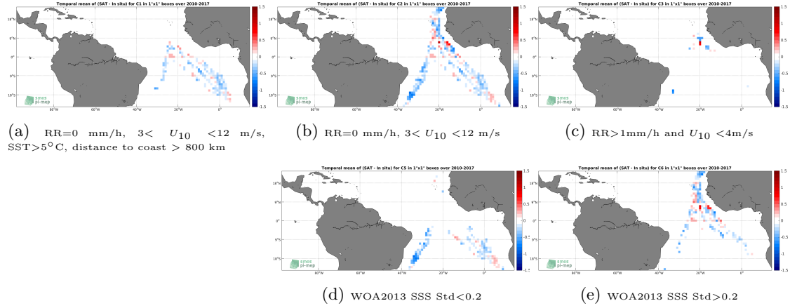
Figure 12: Temporal mean gridded over spatial boxes of size 1^{\circ}\times 1^{\circ} of \Delta\text{SSS} (SMOS L3 v2 - Monthly - 0.25 Deg (CATDS-CECOS-IFREMER) - TSG-POLARSTERN) for 5 different sub-datasets corresponding to:RR=0 mm/h, 3 < U_{10} < 12 m/s, SST >5^{\circ}\text{C} , distance to coast > 800 km (a), RR=0 mm/h, 3 < U_{10} < 12 m/s (b), RR >1 mm/h and U_{10} < 4 m/s (c), WOA2013 SSS Std <0.2 (d), WOA2013 SSS Std >0.2 (e).
