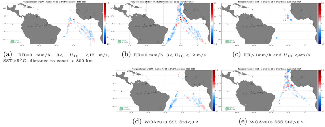
Figure 12: Temporal mean gridded over spatial boxes of size 1^\circ \times 1^\circ of \Delta SSS (SMOS-L3-CATDS-IFREMER-CECOS-V2-MONTHLY-0.25DEG - TSG-POLARSTERN) for 5 different subdatasets corresponding to:RR=0 mm/h, 3 < U_{10} < 12 m/s, SST >5^\circ\text{C} , distance to coast > 800 km (a), RR=0 mm/h, 3 < U_{10} < 12 m/s (b), RR >1 mm/h and U_{10} < 4 m/s (c), WOA2013 SSS Std <0.2 (d), WOA2013 SSS Std >0.2 (e).
