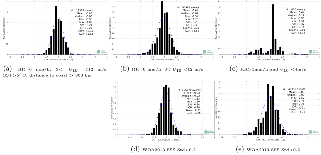
Figure 13: Normalized histogram of \Delta\text{SSS} (SMOS-L3-CATDS-IFREMER-CECOS-V2-MONTHLY-0.25DEG - TSG-POLARSTERN) for 5 different subdatasets corresponding to: RR=0 mm/h, 3 < U_{10} < 12 m/s, SST >5^{\circ}\text{C} , distance to coast > 800 km (a), RR=0 mm/h, 3 < U_{10} < 12 m/s (b), RR>1\text{mm/h} and U_{10} < 4\text{m/s} (c), WOA2013 SSS Std <0.2 (d), WOA2013 SSS Std >0.2 (e).
