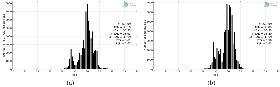
Figure 2: Histograms of SSS from TSG-POLARSTERN (a) and SMOS-L3-CATDS-IFREMER-CECOS-V2-MONTHLY-0.25DEG (b) considering all match-up pairs per bins of 0.1 over the Tropical Atlantic Ocean Pi-MEP region and for the full satellite product period.
