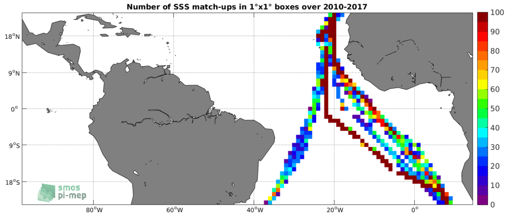
Figure 4: Number of SSS match-ups between TSG-POLARSTERN SSS and the SMOS-L3-CATDS-IFREMER-CECOS-V2-MONTHLY-0.25DEG SSS product for the Tropical Atlantic Ocean Pi-MEP region over 1°x1° boxes and for the full satellite product period.
