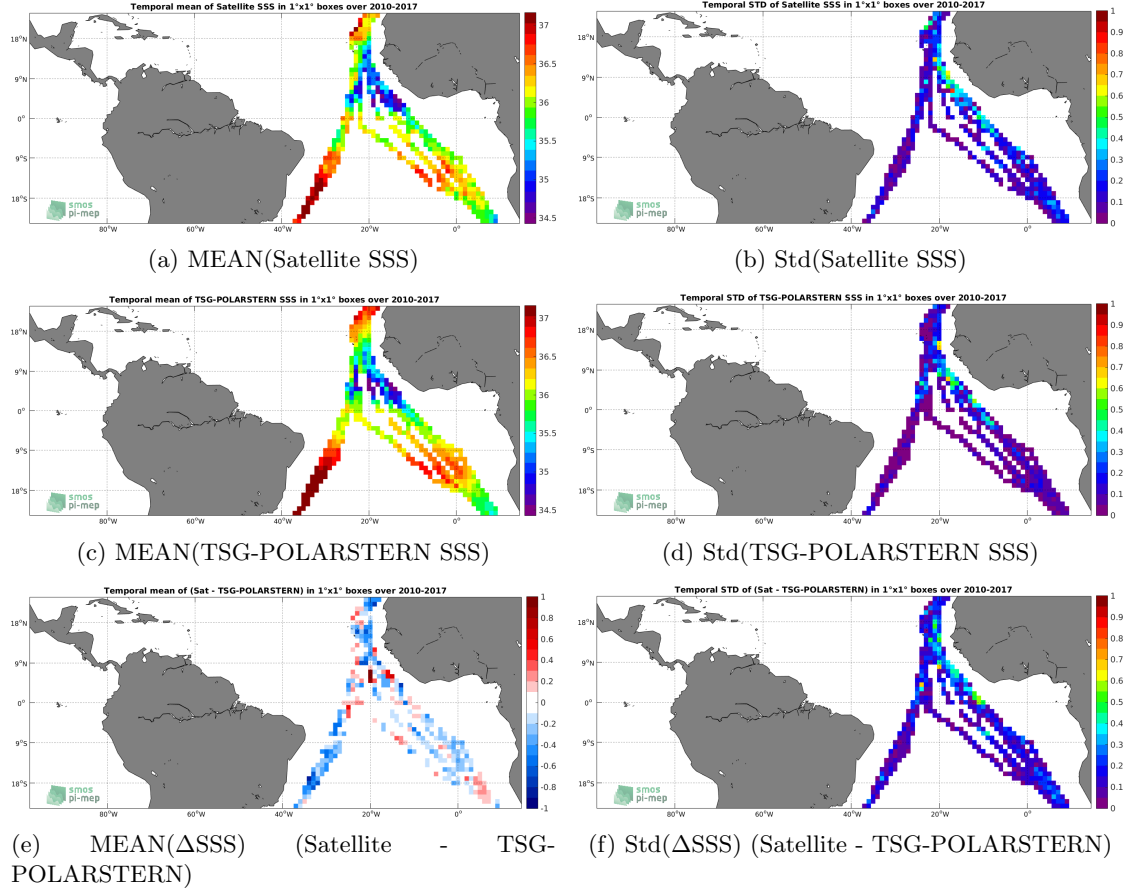
Figure 6: Temporal mean (left) and Std (right) of SSS from SMOS-L3-CATDS-IFREMER-CECOS-V2-MONTHLY-0.25DEG (top), TSG-POLARSTERN (middle), and of \Delta SSS (Satellite - TSG-POLARSTERN). Only match-up pairs are used to generate these maps.
