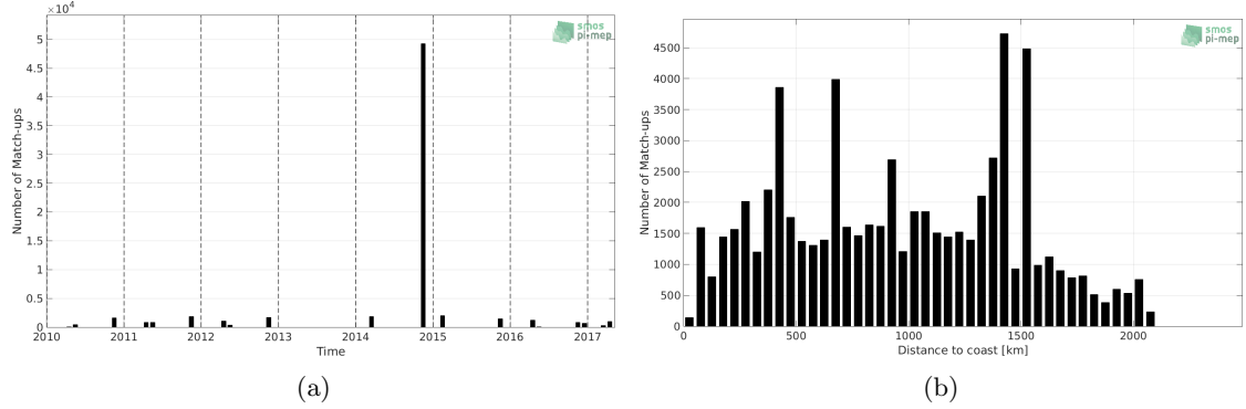
Figure 1: Number of match-ups between TSG-POLARSTERN and SMOS-L3-CATDS-IFREMER-CECOS-V2-MONTHLY-0.25DEG SSS as a function of time (a) and as function of the distance to coast (b) over the Tropical Atlantic Ocean Pi-MEP region and for the full satellite product period.
