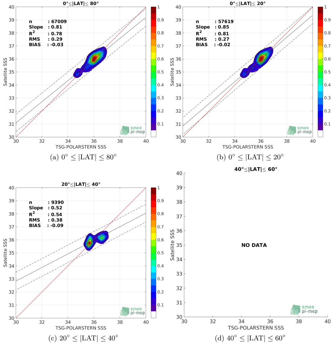
Figure 9: Contour maps of the concentration of SMOS-L3-CATDS-IFREMER-CECOS-V2-MONTHLY-0.25DEG SSS (y-axis) versus TSG-POLARSTERN SSS (x-axis) at match-up pairs for different latitude bands. For each plot, the red line shows x=y . The black thin and dashed lines indicate a linear fit through the data cloud and the \pm 95\% confidence levels, respectively. The number match-up pairs n , the slope and R^2 coefficient of the linear fit, the root mean square (RMS) and the mean bias between satellite and in situ data are indicated for each latitude band in each plots.
