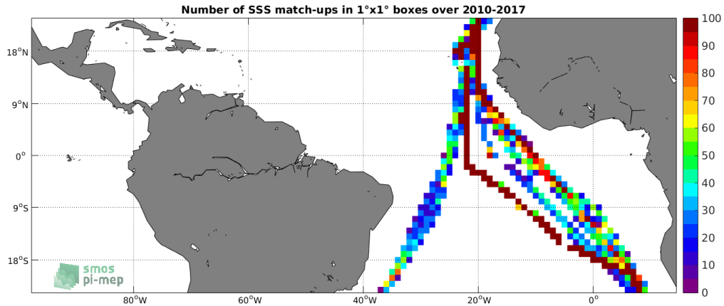
Figure 4: Number of SSS match-ups between TSG-POLARSTERN SSS and the SMOS-L3-CATDS-IFREMER-CECOS-V2-MONTHLY-0.25DEG SSS product for the Tropical Atlantic Ocean Pi-MEP region over 1^\circ \times 1^\circ boxes and for the full satellite product period.
