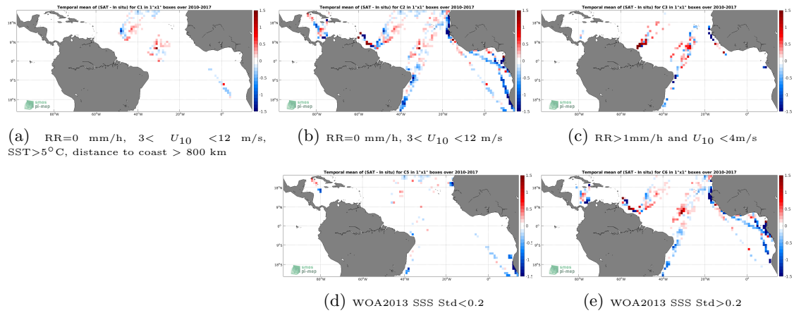
Figure 12: Temporal mean gridded over spatial boxes of size 1^{\circ}\times 1^{\circ} of \Delta\text{SSS} (SMOS SSS L3 v2 - Monthly - 0.25 Deg (CATDS-CECOS-IFREMER) - TSG (LEGOS-DM)) for 5 different subdatasets corresponding to:RR=0 mm/h, 3 < U_{10} < 12 m/s, SST > 5^{\circ}\text{C} , distance to coast > 800 km (a), RR=0 mm/h, 3 < U_{10} < 12 m/s (b), RR > 1 mm/h and U_{10} < 4 m/s (c), WOA2013 SSS Std < 0.2 (d), WOA2013 SSS Std > 0.2 (e).
