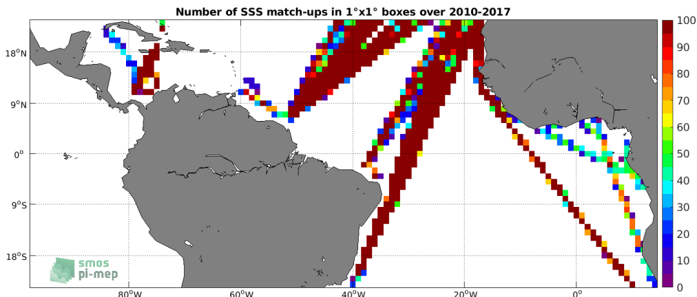
Figure 4: Number of SSS match-ups between TSG (LEGOS-DM) SSS and the SMOS SSS L3 v2 - Monthly - 0.25 Deg (CATDS-CECOS-IFREMER) SSS product for the Tropical Atlantic Ocean Pi-MEP region over 1^\circ \times 1^\circ boxes and for the full satellite product period.
