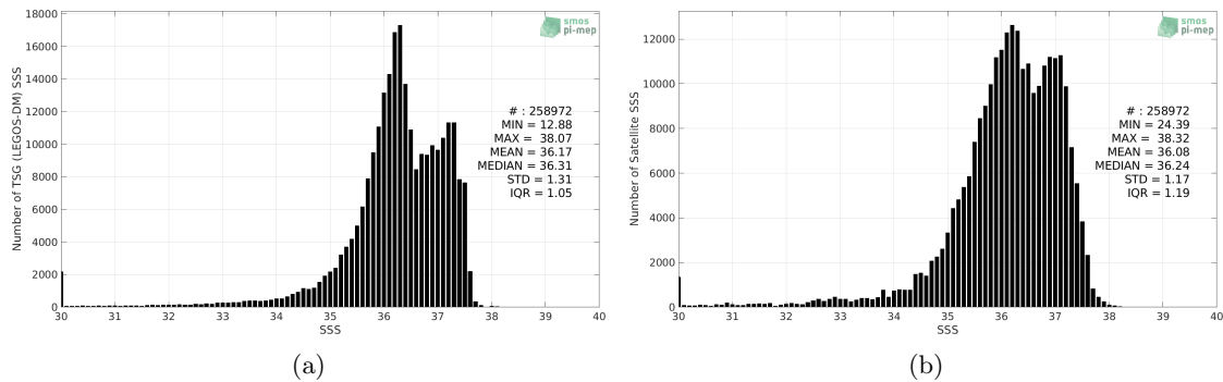
Figure 2: Histograms of SSS from TSG (LEGOS-DM) (a) and SMOS SSS L3 v2 - Monthly - 0.25 Deg (CATDS-CECOS-IFREMER) (b) considering all match-up pairs per bins of 0.1 over the Tropical Atlantic Ocean Pi-MEP region and for the full satellite product period.
