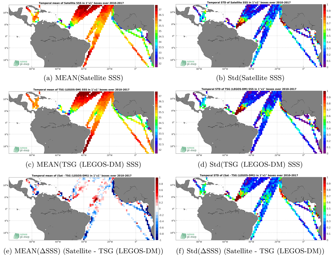
Figure 6: Temporal mean (left) and Std (right) of SSS from SMOS SSS L3 v2 - Monthly - 0.25 Deg (CATDS-CECOS-IFREMER) (top), TSG (LEGOS-DM) (middle), and of \Delta SSS (Satellite - TSG (LEGOS-DM)). Only match-up pairs are used to generate these maps.
