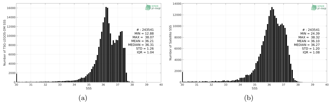
Figure 2: Histograms of SSS from TSG-LEGOS-DM (a) and SMOS L3 v2 - Monthly - 0.25 Deg (CATDS-CECOS-IFREMER) (b) considering all match-up pairs per bins of 0.1 over the Tropical Atlantic Ocean Pi-MEP region and for the full satellite product period.
