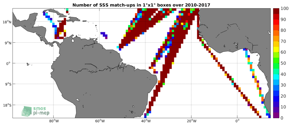
Figure 4: Number of SSS match-ups between TSG-LEGOS-DM SSS and the SMOS L3 v2 - Monthly - 0.25 Deg (CATDS-CECOS-IFREMER) SSS product for the Tropical Atlantic Ocean Pi-MEP region over 1^\circ \times 1^\circ boxes and for the full satellite product period.
