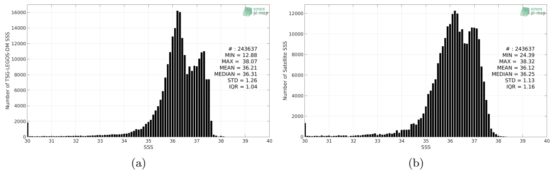
Figure 2: Histograms of SSS from TSG-LEGOS-DM (a) and SMOS-L3-CATDS-IFREMER-CECOS-V2-MONTHLY-0.25DEG (b) considering all match-up pairs per bins of 0.1 over the Tropical Atlantic Ocean Pi-MEP region and for the full satellite product period.
