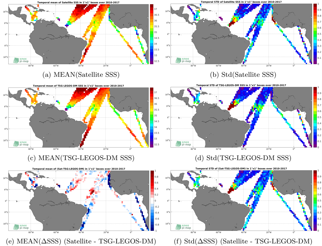
Figure 6: Temporal mean (left) and Std (right) of SSS from SMOS-L3-CATDS-IFREMER-CECOS-V2-MONTHLY-0.25DEG (top), TSG-LEGOS-DM (middle), and of \Delta SSS (Satellite - TSG-LEGOS-DM). Only match-up pairs are used to generate these maps.
