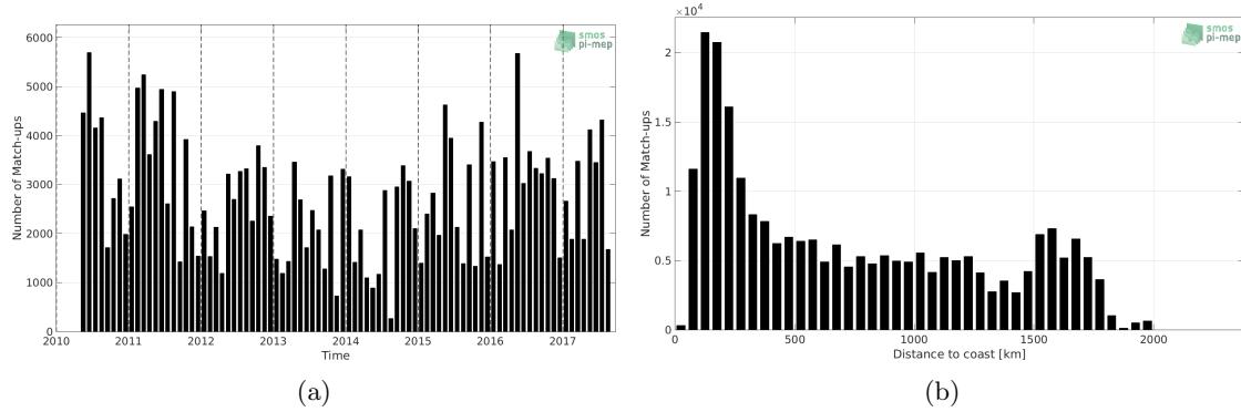
Figure 1: Number of match-ups between TSG-LEGOS-DM and SMOS-L3-CATDS-IFREMER-CECOS-V2-MONTHLY-0.25DEG SSS as a function of time (a) and as function of the distance to coast (b) over the Tropical Atlantic Ocean Pi-MEP region and for the full satellite product period.
