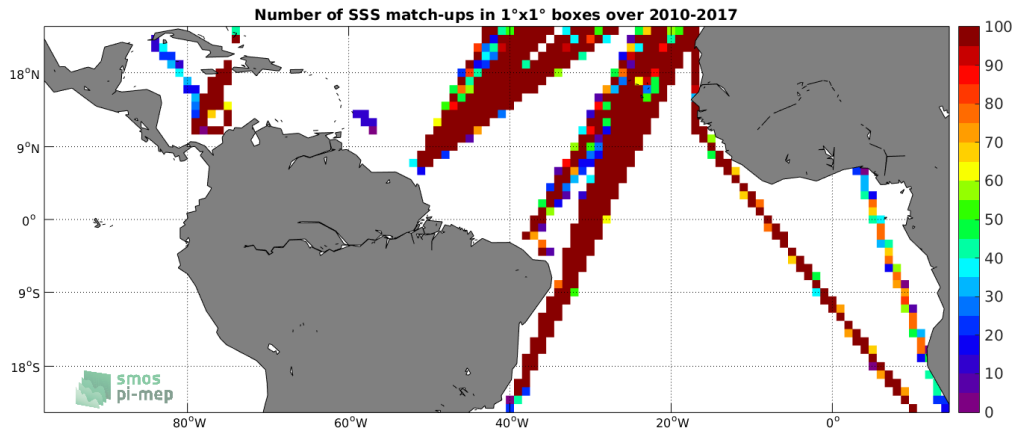
Figure 4: Number of SSS match-ups between TSG-LEGOS-DM SSS and the SMOS-L3-CATDS-IFREMER-CECOS-V2-MONTHLY-0.25DEG SSS product for the Tropical Atlantic Ocean Pi-MEP region over 1^\circ \times 1^\circ boxes and for the full satellite product period.
