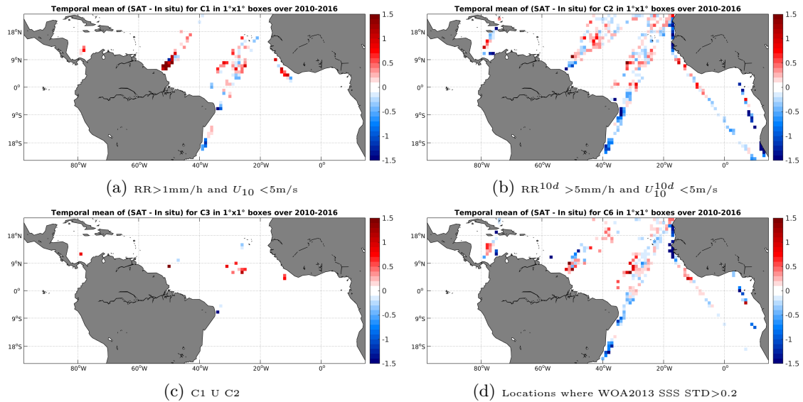
Figure 12: Temporal mean gridded over spatial boxes of size 1^\circ \times 1^\circ of \Delta SSS (SMOS-L3-CATDS-IFREMER-CECOS-V2-MONTHLY-0.25DEG - TSG-LEGOS-DM) for 4 different subdatasets corresponding to:RR>1mm/h and U_{10} < 5\text{m/s} (a), RR^{10d} > 5\text{mm/h} and U_{10}^{10d} < 5\text{m/s} (b), C1 U C2 (c),Locations where WOA2013 SSS STD>0.2 (d).
