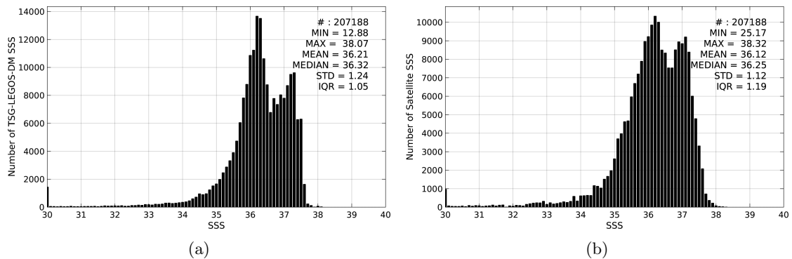
Figure 2: Histograms of SSS from TSG-LEGOS-DM (a) and SMOS-L3-CATDS-IFREMER-CECOS-V2-MONTHLY-0.25DEG (b) considering all match-up pairs per bins of 0.1 over the Tropical Atlantic Ocean Pi-MEP region and for the full satellite product period.
