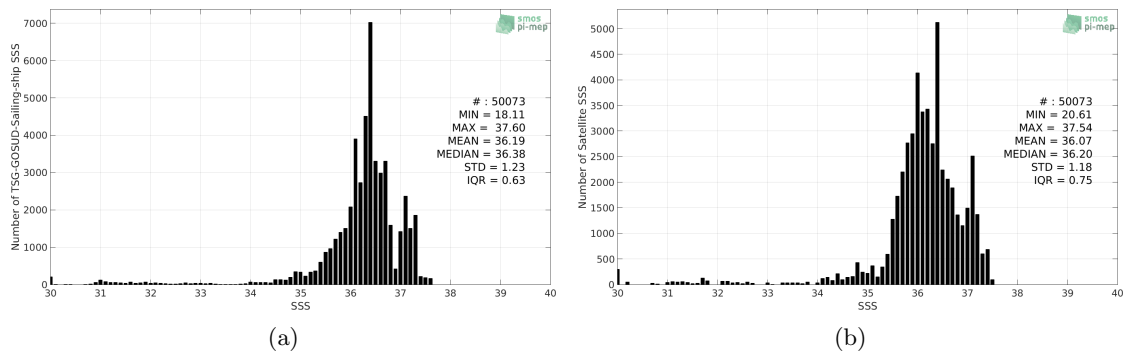
Figure 2: Histograms of SSS from TSG-GOSUD-Sailing-ship (a) and SMOS L3 v2 - Monthly - 0.25 Deg (CATDS-CECOS-IFREMER) (b) considering all match-up pairs per bins of 0.1 over the Tropical Atlantic Ocean Pi-MEP region and for the full satellite product period.
