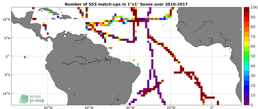
Figure 4: Number of SSS match-ups between TSG-GOSUD-Sailing-ship SSS and the SMOS L3 v2 - Monthly - 0.25 Deg (CATDS-CECOS-IFREMER) SSS product for the Tropical Atlantic Ocean Pi-MEP region over 1^\circ \times 1^\circ boxes and for the full satellite product period.
