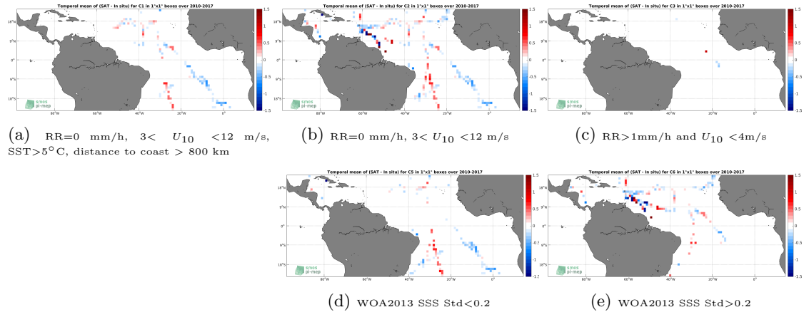
Figure 12: Temporal mean gridded over spatial boxes of size 1^{\circ}\times 1^{\circ} of \Delta SSS (SMOS L3 v2 - Monthly - 0.25 Deg (CATDS-CECOS-IFREMER) - TSG-GOSUD-Sailing-ship) for 5 different subdatasets corresponding to:RR=0 mm/h, 3 < U_{10} < 12 m/s, SST >5^{\circ}\text{C} , distance to coast > 800 km (a), RR=0 mm/h, 3 < U_{10} < 12 m/s (b), RR >1 mm/h and U_{10} < 4 m/s (c), WOA2013 SSS Std <0.2 (d), WOA2013 SSS Std >0.2 (e).
