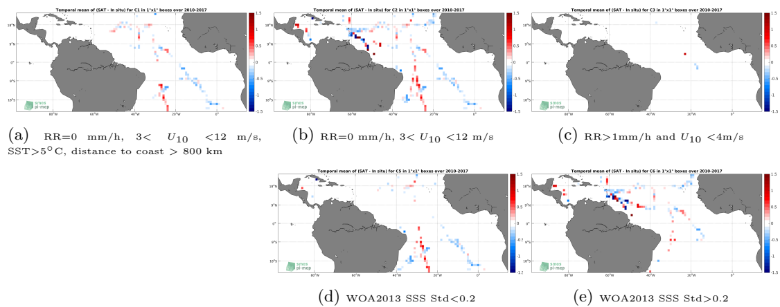
Figure 12: Temporal mean gridded over spatial boxes of size 1^\circ \times 1^\circ of \Delta\text{SSS} (SMOS-L3-CATDS-IFREMER-CECOS-V2-MONTHLY-0.25DEG - TSG-GOSUD-Sailing-ship) for 5 different sub-datasets corresponding to:RR=0 mm/h, 3 < U_{10} < 12 m/s, SST>5°C, distance to coast > 800 km (a), RR=0 mm/h, 3 < U_{10} < 12 m/s (b), RR>1mm/h and U_{10} < 4 m/s (c), WOA2013 SSS Std<0.2 (d), WOA2013 SSS Std>0.2 (e).
