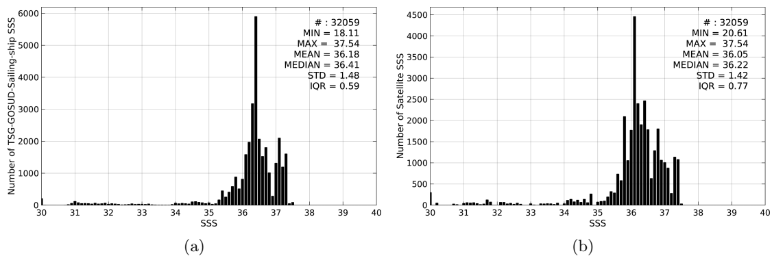
Figure 2: Histograms of SSS from TSG-GOSUD-Sailing-ship (a) and SMOS-L3-CATDS-IFREMER-CECOS-V2-MONTHLY-0.25DEG (b) considering all match-up pairs per bins of 0.1 over the Tropical Atlantic Ocean Pi-MEP region and for the full satellite product period.
