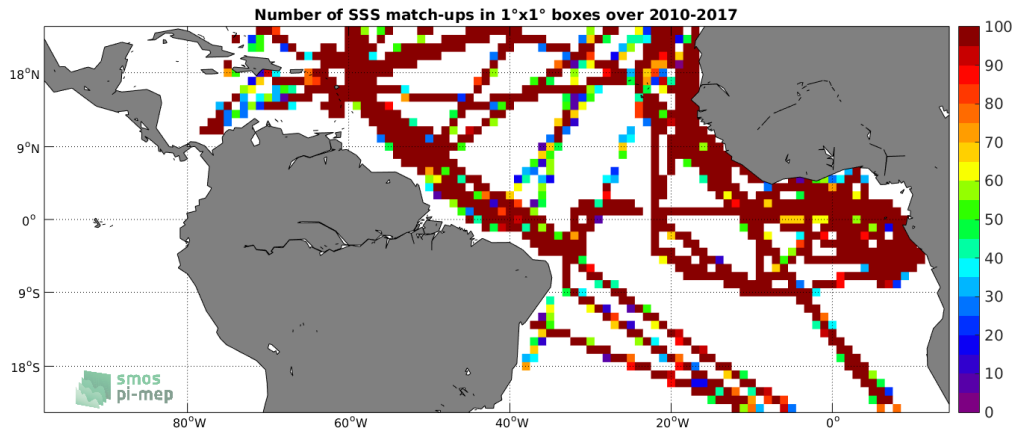
Figure 4: Number of SSS match-ups between TSG-GOSUD-Research-vessel SSS and the SMOS L3 v2 - Monthly - 0.25 Deg (CATDS-CECOS-IFREMER) SSS product for the Tropical Atlantic Ocean Pi-MEP region over 1°x1° boxes and for the full satellite product period.
