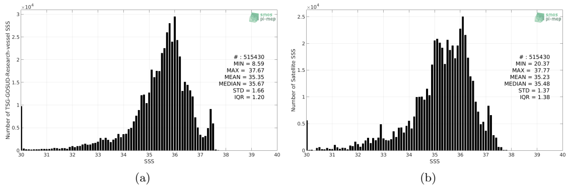
Figure 2: Histograms of SSS from TSG-GOSUD-Research-vessel (a) and SMOS L3 v2 - Monthly - 0.25 Deg (CATDS-CECOS-IFREMER) (b) considering all match-up pairs per bins of 0.1 over the Tropical Atlantic Ocean Pi-MEP region and for the full satellite product period.
