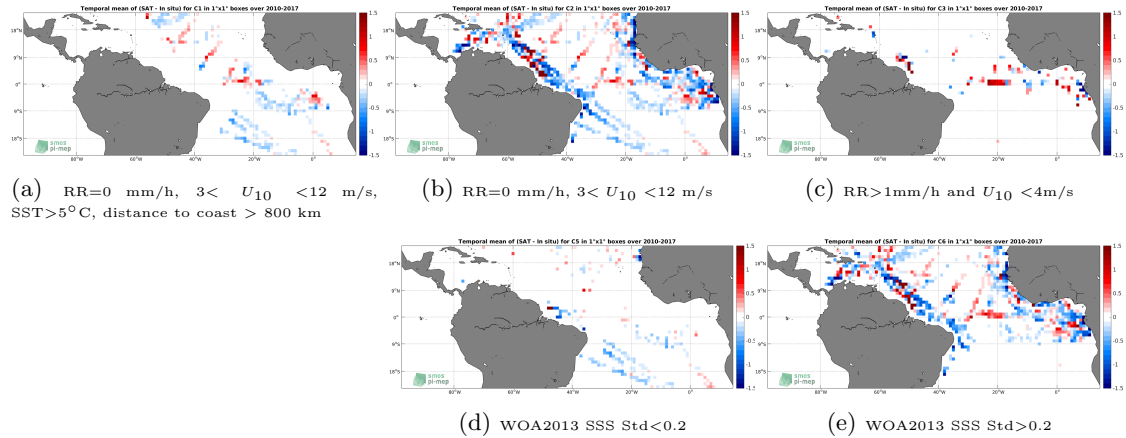
Figure 12: Temporal mean gridded over spatial boxes of size 1^{\circ}\times 1^{\circ} of \Delta SSS (SMOS L3 v2 - Monthly - 0.25 Deg (CATDS-CECOS-IFREMER) - TSG-GOSUD-Research-vessel) for 5 different subdatasets corresponding to:RR=0 mm/h, 3 < U_{10} < 12 m/s, SST > 5^{\circ}\text{C} , distance to coast > 800 km (a), RR=0 mm/h, 3 < U_{10} < 12 m/s (b), RR > 1 mm/h and U_{10} < 4 m/s (c), WOA2013 SSS Std < 0.2 (d), WOA2013 SSS Std > 0.2 (e).
