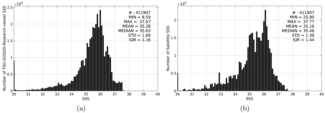
Figure 2: Histograms of SSS from TSG-GOSUD-Research-vessel (a) and SMOS-L3-CATDS-IFREMER-CECOS-V2-MONTHLY-0.25DEG (b) considering all match-up pairs per bins of 0.1 over the Tropical Atlantic Ocean Pi-MEP region and for the full satellite product period.
