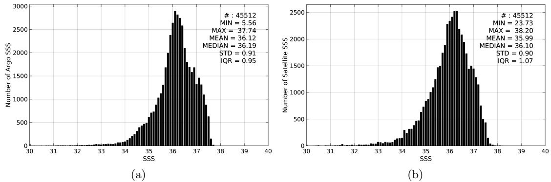
Figure 2: Histograms of SSS from Argo (a) and SMOS-L3-CATDS-IFREMER-CECOS-V2-MONTHLY-0.25DEG (b) considering all match-up pairs per bins of 0.1 over the Tropical Atlantic Ocean Pi-MEP region and for the full satellite product period.
