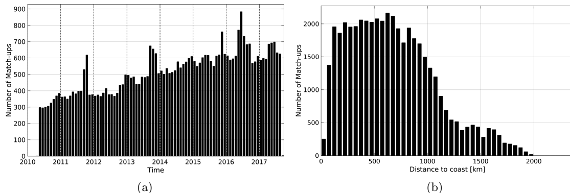
Figure 1: Number of match-ups between Argo and SMOS-L3-CATDS-IFREMER-CECOS-V2-MONTHLY-0.25DEG SSS as a function of time (a) and as function of the distance to coast (b) over the Tropical Atlantic Ocean Pi-MEP region and for the full satellite product period.
