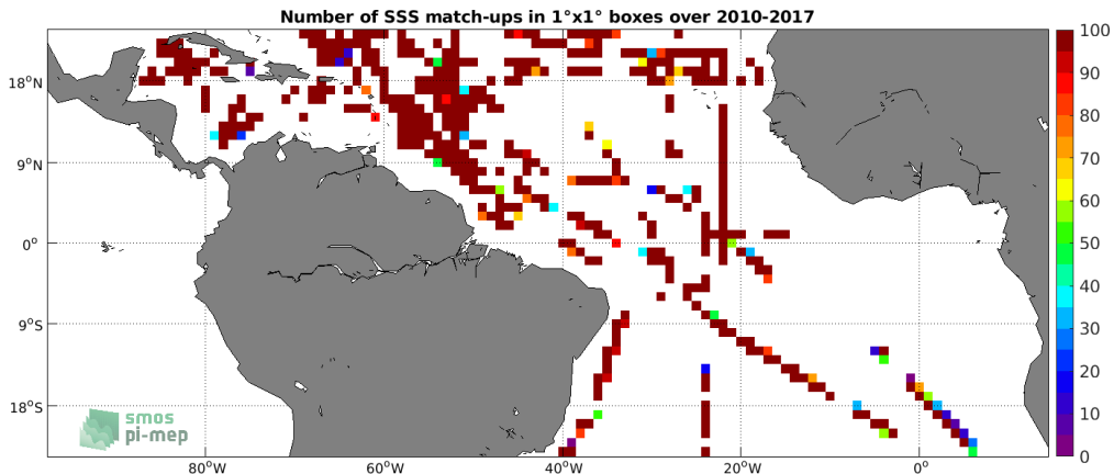
Figure 4: Number of SSS match-ups between TSG (SAMOS) SSS and the SMOS SSS L3 v2 - Daily - 0.5 Deg (CATDS-CECOS-IFREMER) SSS product for the Tropical Atlantic Ocean Pi-MEP region over 1^\circ \times 1^\circ boxes and for the full satellite product period.
