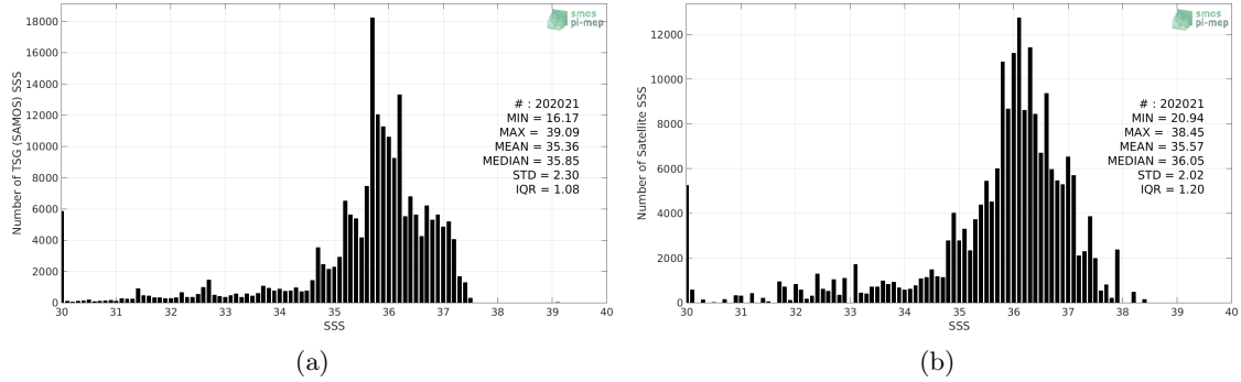
Figure 2: Histograms of SSS from TSG (SAMOS) (a) and SMOS SSS L3 v2 - Daily - 0.5 Deg (CATDS-CECOS-IFREMER) (b) considering all match-up pairs per bins of 0.1 over the Tropical Atlantic Ocean Pi-MEP region and for the full satellite product period.
