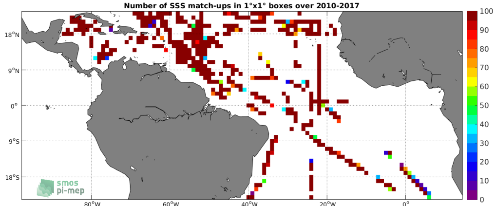
Figure 4: Number of SSS match-ups between TSG (SAMOS) SSS and the SMOS SSS L3 v2 - Daily - 0.5 Deg (CATDS-CECOS-IFREMER) SSS product for the Tropical Atlantic Ocean Pi-MEP region over 1^\circ \times 1^\circ boxes and for the full satellite product period.
