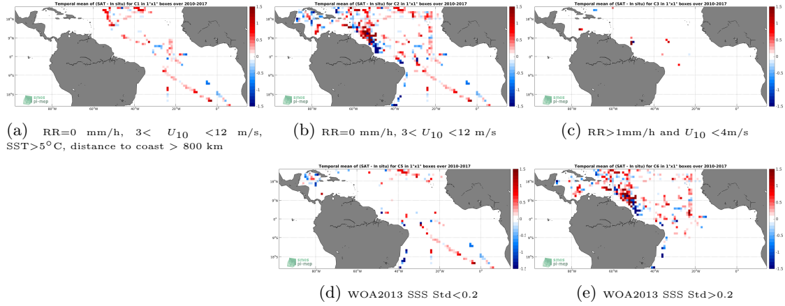
Figure 12: Temporal mean gridded over spatial boxes of size 1^{\circ}\times 1^{\circ} of \Delta\text{SSS} (SMOS SSS L3 v2 - Daily - 0.5 Deg (CATDS-CECOS-IFREMER) - TSG (SAMOS)) for 5 different subdatasets corresponding to:RR=0 mm/h, 3 < U_{10} < 12 m/s, SST >5^{\circ}\text{C} , distance to coast > 800 km (a), RR=0 mm/h, 3 < U_{10} < 12 m/s (b), RR >1 mm/h and U_{10} < 4 m/s (c), WOA2013 SSS Std <0.2 (d), WOA2013 SSS Std >0.2 (e).
