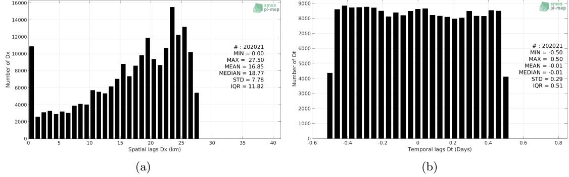
Figure 5: Histograms of the spatial (a) and temporal (b) lags between the time of the TSG (SAMOS) measurements and the date of the corresponding SMOS SSS L3 v2 - Daily - 0.5 Deg (CATDS-CECOS-IFREMER) SSS product.
