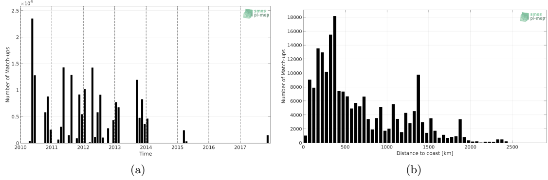
Figure 1: Number of match-ups between TSG (SAMOS) and SMOS SSS L3 v2 - Daily - 0.5 Deg (CATDS-CECOS-IFREMER) SSS as a function of time (a) and as function of the distance to coast (b) over the Tropical Atlantic Ocean Pi-MEP region and for the full satellite product period.
