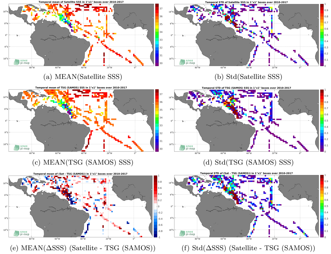
Figure 6: Temporal mean (left) and Std (right) of SSS from SMOS SSS L3 v2 - Daily - 0.5 Deg (CATDS-CECOS-IFREMER) (top), TSG (SAMOS) (middle), and of \Delta SSS (Satellite - TSG (SAMOS)). Only match-up pairs are used to generate these maps.
