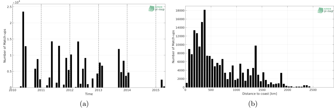
Figure 1: Number of match-ups between TSG-SAMOS and SMOS L3 v2 - Daily - 0.5 Deg (CATDS-CECOS-IFREMER) SSS as a function of time (a) and as function of the distance to coast (b) over the Tropical Atlantic Ocean Pi-MEP region and for the full satellite product period.
