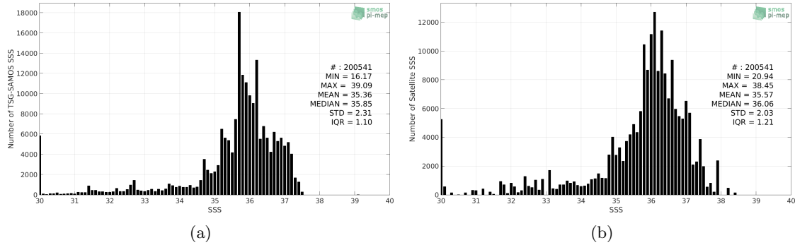
Figure 2: Histograms of SSS from TSG-SAMOS (a) and SMOS L3 v2 - Daily - 0.5 Deg (CATDS-CECOS-IFREMER) (b) considering all match-up pairs per bins of 0.1 over the Tropical Atlantic Ocean Pi-MEP region and for the full satellite product period.
