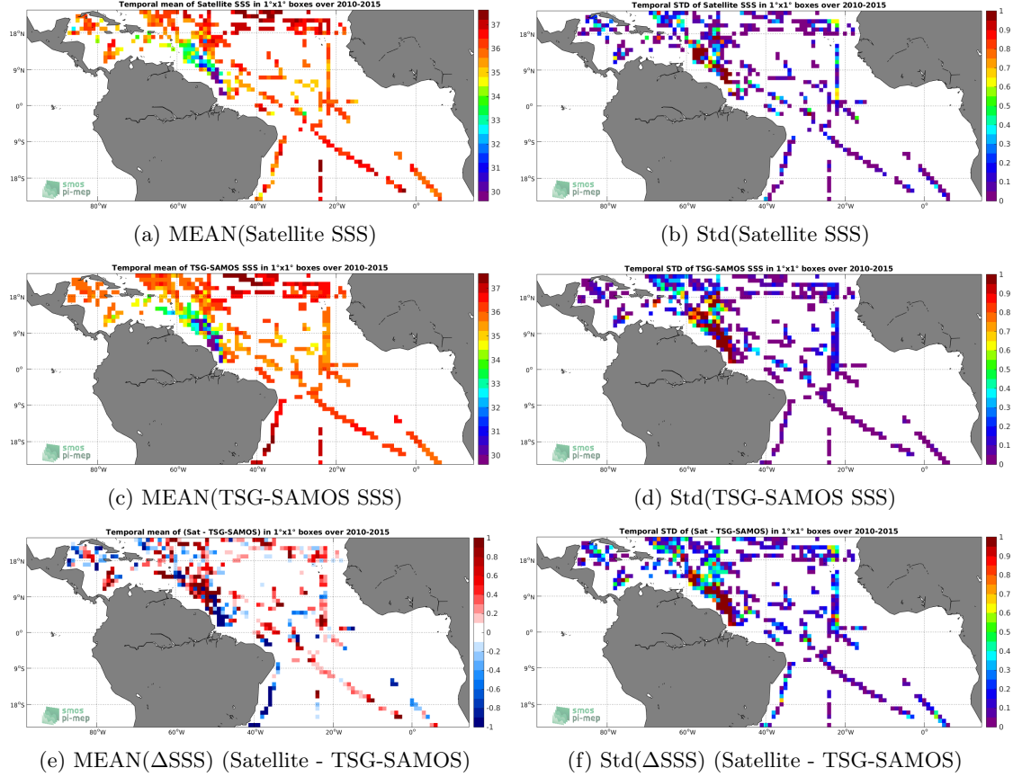
Figure 6: Temporal mean (left) and Std (right) of SSS from SMOS L3 v2 - Daily - 0.5 Deg (CATDS-CECOS-IFREMER) (top), TSG-SAMOS (middle), and of \Delta SSS (Satellite - TSG-SAMOS). Only match-up pairs are used to generate these maps.
