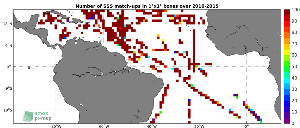
Figure 4: Number of SSS match-ups between TSG-SAMOS SSS and the SMOS L3 v2 - Daily - 0.5 Deg (CATDS-CECOS-IFREMER) SSS product for the Tropical Atlantic Ocean Pi-MEP region over 1°x1° boxes and for the full satellite product period.
