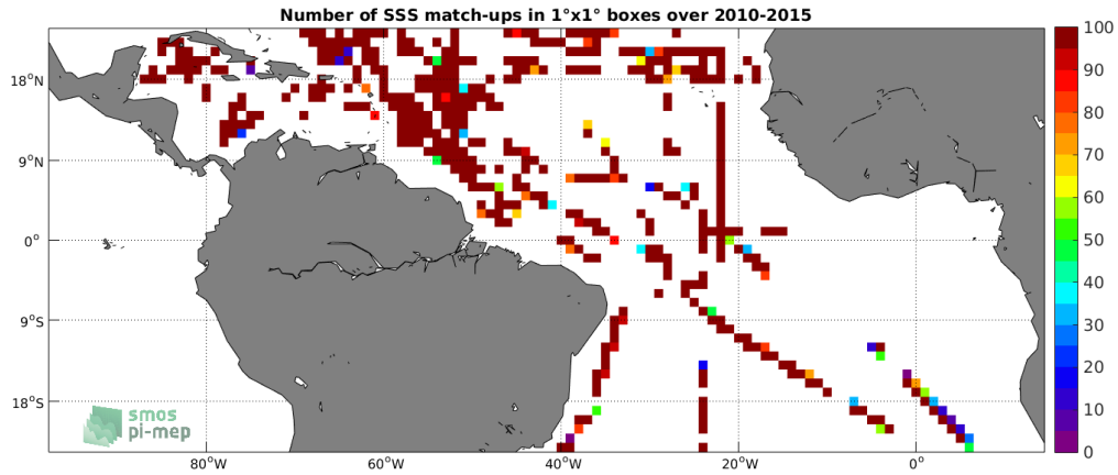
Figure 4: Number of SSS match-ups between TSG-SAMOS SSS and the SMOS-L3-CATDS-CECOS-IFREMER-V2-1DAY-0.5DEG SSS product for the Tropical Atlantic Ocean Pi-MEP region over 1°x1° boxes and for the full satellite product period.
