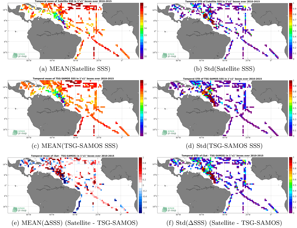
Figure 6: Temporal mean (left) and Std (right) of SSS from SMOS-L3-CATDS-CECOS-IFREMER-V2-1DAY-0.5DEG (top), TSG-SAMOS (middle), and of \Delta SSS (Satellite - TSG-SAMOS). Only match-up pairs are used to generate these maps.
