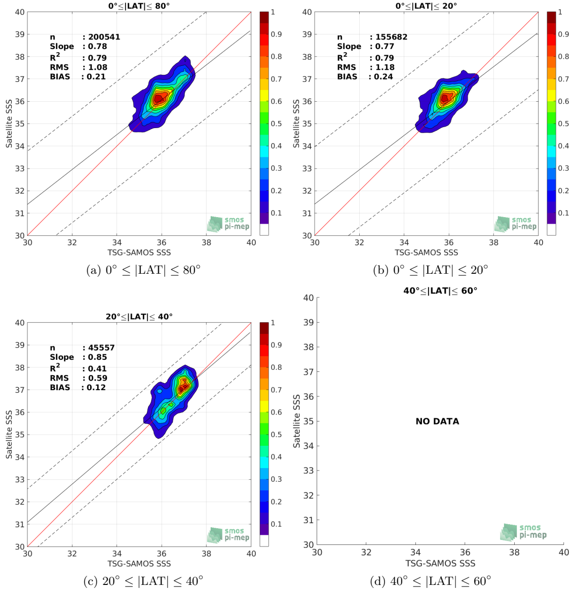
Figure 9: Contour maps of the concentration of SMOS-L3-CATDS-CECOS-IFREMER-V2-1DAY-0.5DEG SSS (y-axis) versus TSG-SAMOS SSS (x-axis) at match-up pairs for different latitude bands. For each plot, the red line shows x=y . The black thin and dashed lines indicate a linear fit through the data cloud and the \pm 95\% confidence levels, respectively. The number match-up pairs n , the slope and R^2 coefficient of the linear fit, the root mean square (RMS) and the mean bias between satellite and in situ data are indicated for each latitude band in each plots.
