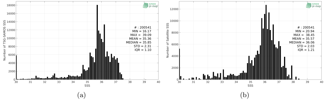
Figure 2: Histograms of SSS from TSG-SAMOS (a) and SMOS-L3-CATDS-CECOS-IFREMER-V2-1DAY-0.5DEG (b) considering all match-up pairs per bins of 0.1 over the Tropical Atlantic Ocean Pi-MEP region and for the full satellite product period.
