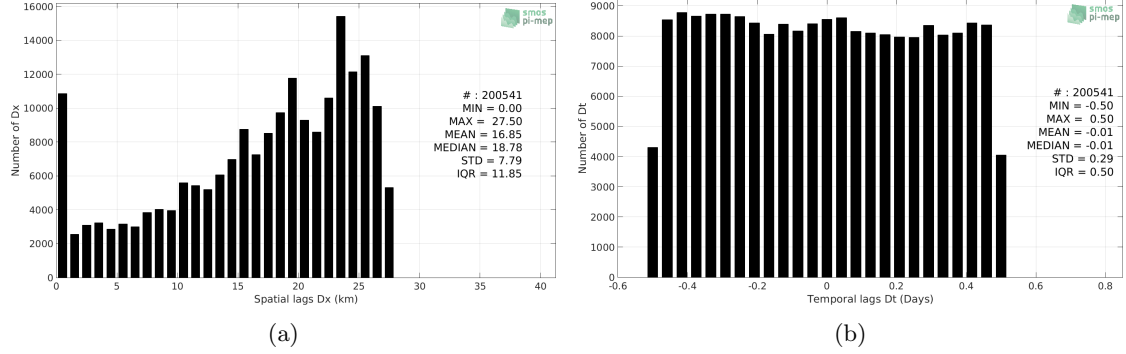
Figure 5: Histograms of the spatial (a) and temporal (b) lags between the time of the TSG-SAMOS measurements and the date of the corresponding SMOS-L3-CATDS-CECOS-IFREMER-V2-1DAY-0.5DEG SSS product.
