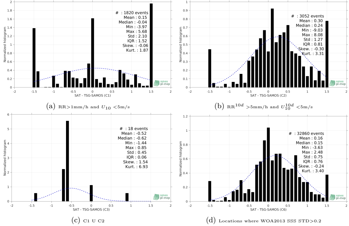
Figure 13: Normalized histogram of \Delta\text{SSS} (SMOS-L3-CATDS-CECOS-IFREMER-V2-1DAY-0.5DEG - TSG-SAMOS) for 6 different subdatasets corresponding to: RR>1mm/h and U_{10} < 5\text{m/s} (a), RR^{10d} > 5\text{mm/h} and U_{10}^{10d} < 5\text{m/s} (b), C1 U C2 (c), Locations where WOA2013 SSS STD>0.2 (d).
