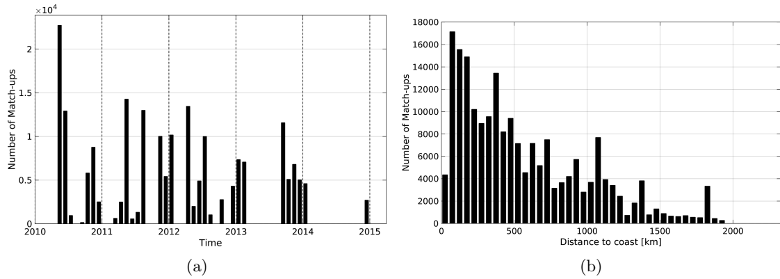
Figure 1: Number of match-ups between TSG-SAMOS and SMOS-L3-CATDS-CECOS-IFREMER-V2-1DAY-0.5deg SSS as a function of time (a) and as function of the distance to coast (b) over the Tropical Atlantic Ocean Pi-MEP region and for the full satellite product period.
