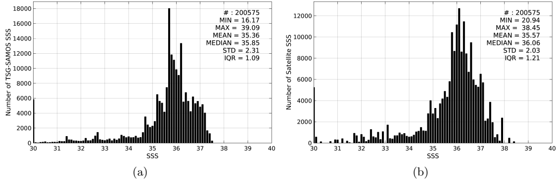
Figure 2: Histograms of SSS from TSG-SAMOS (a) and SMOS-L3-CATDS-CECOS-IFREMER-V2-1DAY-0.5deg (b) considering all match-up pairs per bins of 0.1 over the Tropical Atlantic Ocean Pi-MEP region and for the full satellite product period.
