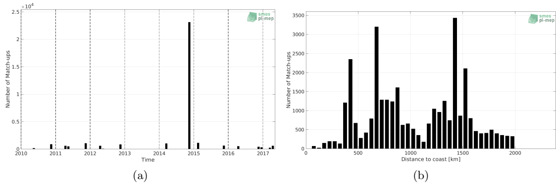
Figure 1: Number of match-ups between TSG (Polarstern) and SMOS SSS L3 v2 - Daily - 0.5 Deg (CATDS-CECOS-IFREMER) SSS as a function of time (a) and as function of the distance to coast (b) over the Tropical Atlantic Ocean Pi-MEP region and for the full satellite product period.
