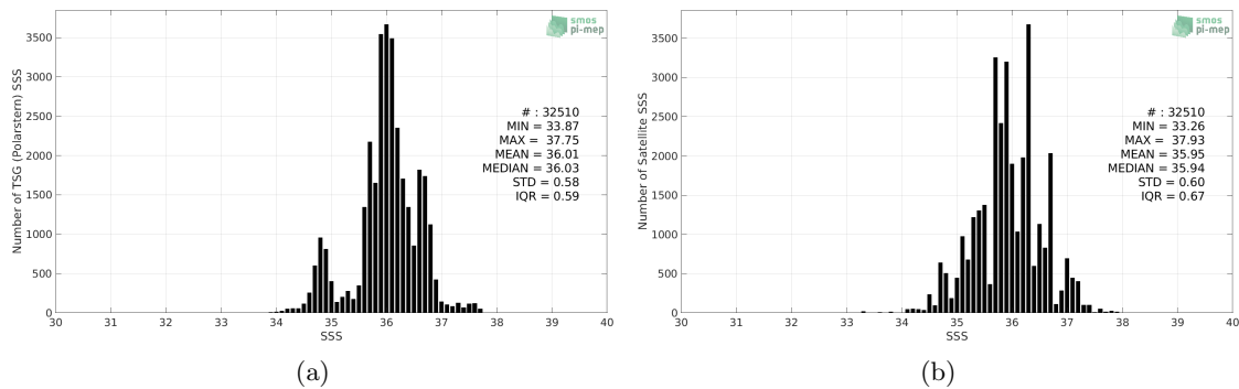
Figure 2: Histograms of SSS from TSG (Polarstern) (a) and SMOS SSS L3 v2 - Daily - 0.5 Deg (CATDS-CECOS-IFREMER) (b) considering all match-up pairs per bins of 0.1 over the Tropical Atlantic Ocean Pi-MEP region and for the full satellite product period.
