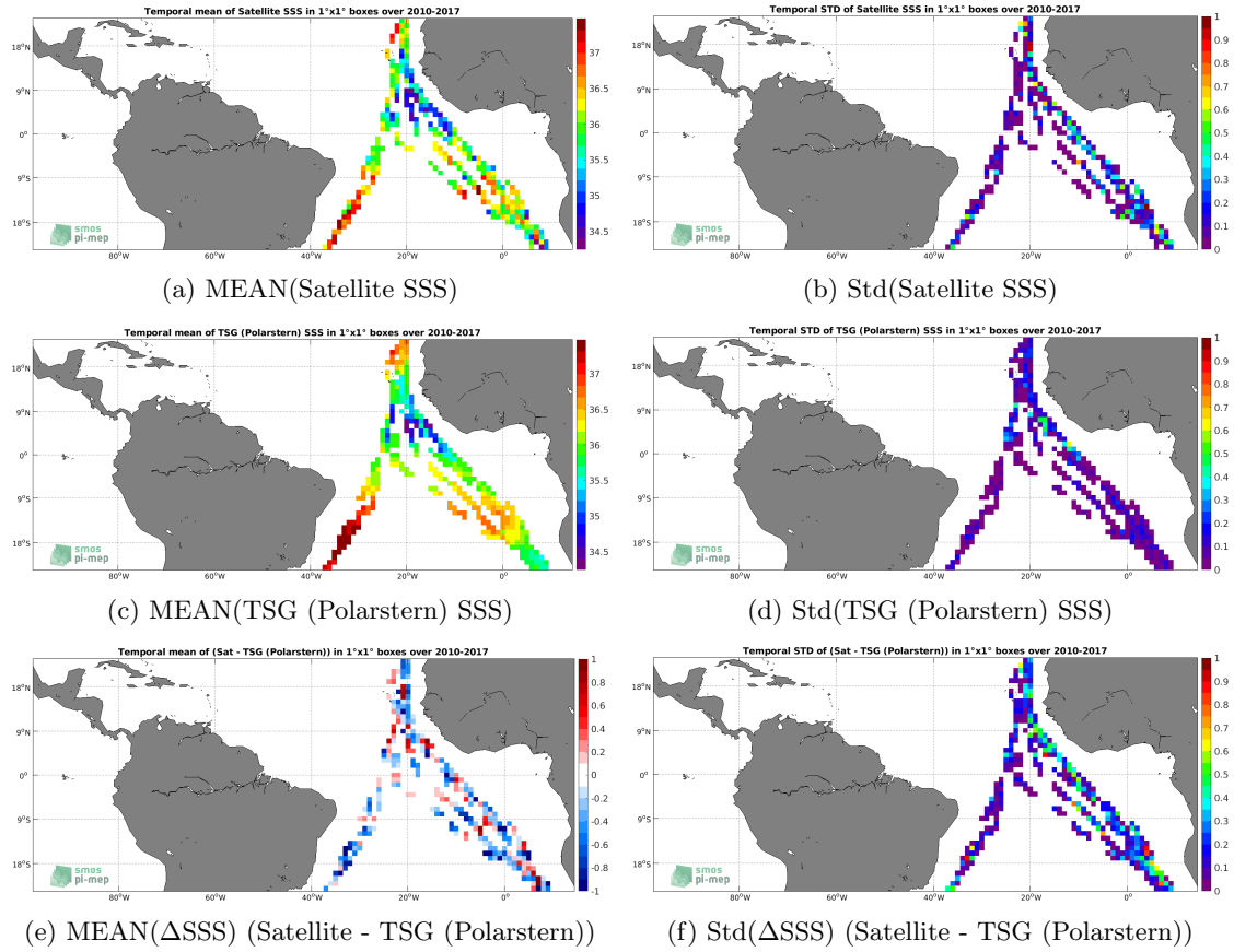
Figure 6: Temporal mean (left) and Std (right) of SSS from SMOS SSS L3 v2 - Daily - 0.5 Deg (CATDS-CECOS-IFREMER) (top), TSG (Polarstern) (middle), and of \Delta SSS (Satellite - TSG (Polarstern)). Only match-up pairs are used to generate these maps.
