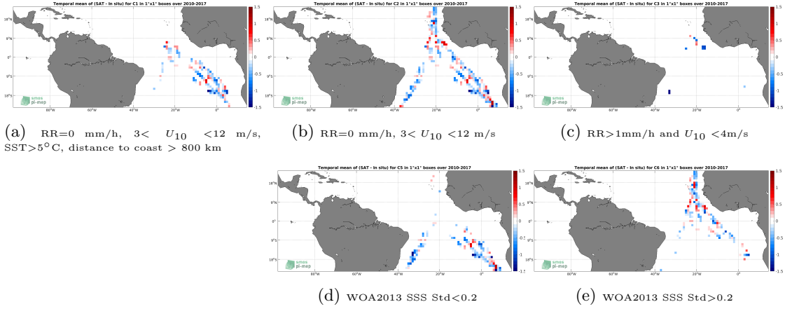
Figure 12: Temporal mean gridded over spatial boxes of size 1^{\circ}\times 1^{\circ} of \Delta\text{SSS} (SMOS SSS L3 v2 - Daily - 0.5 Deg (CATDS-CECOS-IFREMER) - TSG (Polarstern)) for 5 different subdatasets corresponding to:RR=0 mm/h, 3 < U_{10} < 12 m/s, SST > 5^{\circ}\text{C} , distance to coast > 800 km (a), RR=0 mm/h, 3 < U_{10} < 12 m/s (b), RR > 1 mm/h and U_{10} < 4 m/s (c), WOA2013 SSS Std < 0.2 (d), WOA2013 SSS Std > 0.2 (e).
