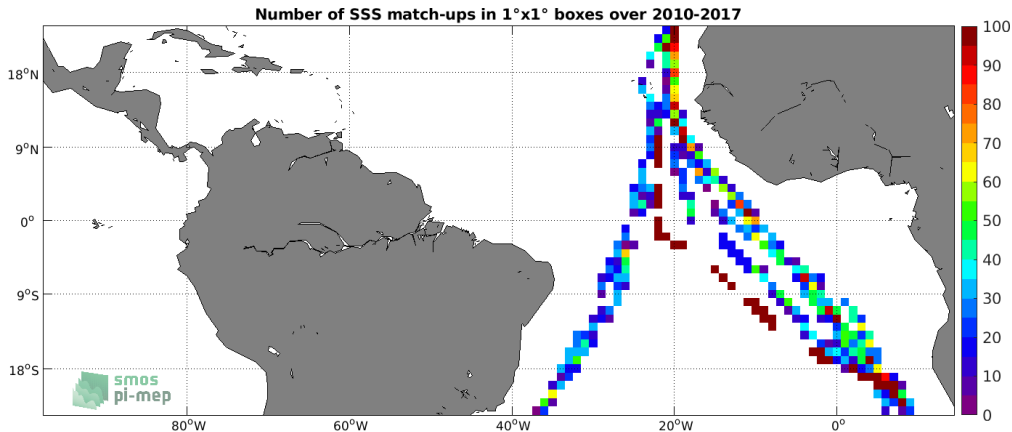
Figure 4: Number of SSS match-ups between TSG (Polarstern) SSS and the SMOS SSS L3 v2 - Daily - 0.5 Deg (CATDS-CECOS-IFREMER) SSS product for the Tropical Atlantic Ocean Pi-MEP region over 1^\circ \times 1^\circ boxes and for the full satellite product period.
