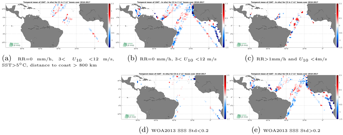
Figure 12: Temporal mean gridded over spatial boxes of size 1^{\circ}\times 1^{\circ} of \Delta\text{SSS} (SMOS SSS L3 v2 - Daily - 0.5 Deg (CATDS-CECOS-IFREMER) - TSG (LEGOS-DM)) for 5 different subdatasets corresponding to:RR=0 mm/h, 3 < U_{10} < 12 m/s, SST > 5^{\circ}\text{C} , distance to coast > 800 km (a), RR=0 mm/h, 3 < U_{10} < 12 m/s (b), RR > 1 mm/h and U_{10} < 4 m/s (c), WOA2013 SSS Std < 0.2 (d), WOA2013 SSS Std > 0.2 (e).
