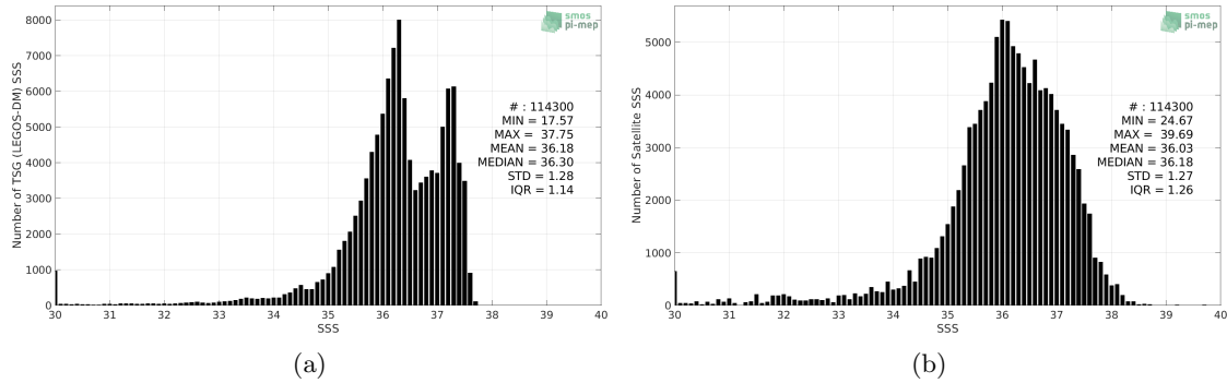
Figure 2: Histograms of SSS from TSG (LEGOS-DM) (a) and SMOS SSS L3 v2 - Daily - 0.5 Deg (CATDS-CECOS-IFREMER) (b) considering all match-up pairs per bins of 0.1 over the Tropical Atlantic Ocean Pi-MEP region and for the full satellite product period.
