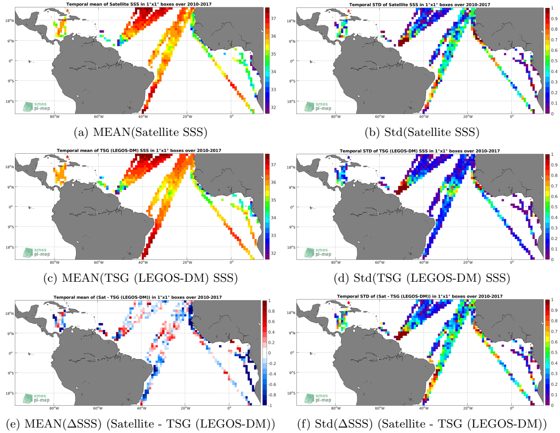
Figure 6: Temporal mean (left) and Std (right) of SSS from SMOS SSS L3 v2 - Daily - 0.5 Deg (CATDS-CECOS-IFREMER) (top), TSG (LEGOS-DM) (middle), and of \Delta SSS (Satellite - TSG (LEGOS-DM)). Only match-up pairs are used to generate these maps.
