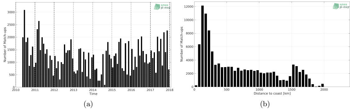
Figure 1: Number of match-ups between TSG (LEGOS-DM) and SMOS SSS L3 v2 - Daily - 0.5 Deg (CATDS-CECOS-IFREMER) SSS as a function of time (a) and as function of the distance to coast (b) over the Tropical Atlantic Ocean Pi-MEP region and for the full satellite product period.
