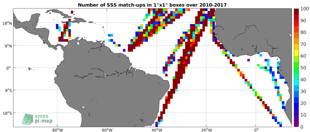
Figure 4: Number of SSS match-ups between TSG (LEGOS-DM) SSS and the SMOS SSS L3 v2 - Daily - 0.5 Deg (CATDS-CECOS-IFREMER) SSS product for the Tropical Atlantic Ocean Pi-MEP region over 1^\circ \times 1^\circ boxes and for the full satellite product period.
