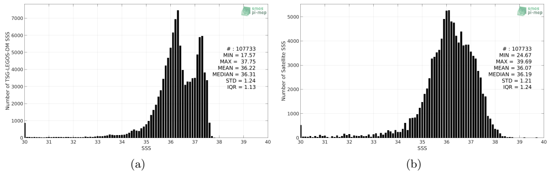
Figure 2: Histograms of SSS from TSG-LEGOS-DM (a) and SMOS L3 v2 - Daily - 0.5 Deg (CATDS-CECOS-IFREMER) (b) considering all match-up pairs per bins of 0.1 over the Tropical Atlantic Ocean Pi-MEP region and for the full satellite product period.
