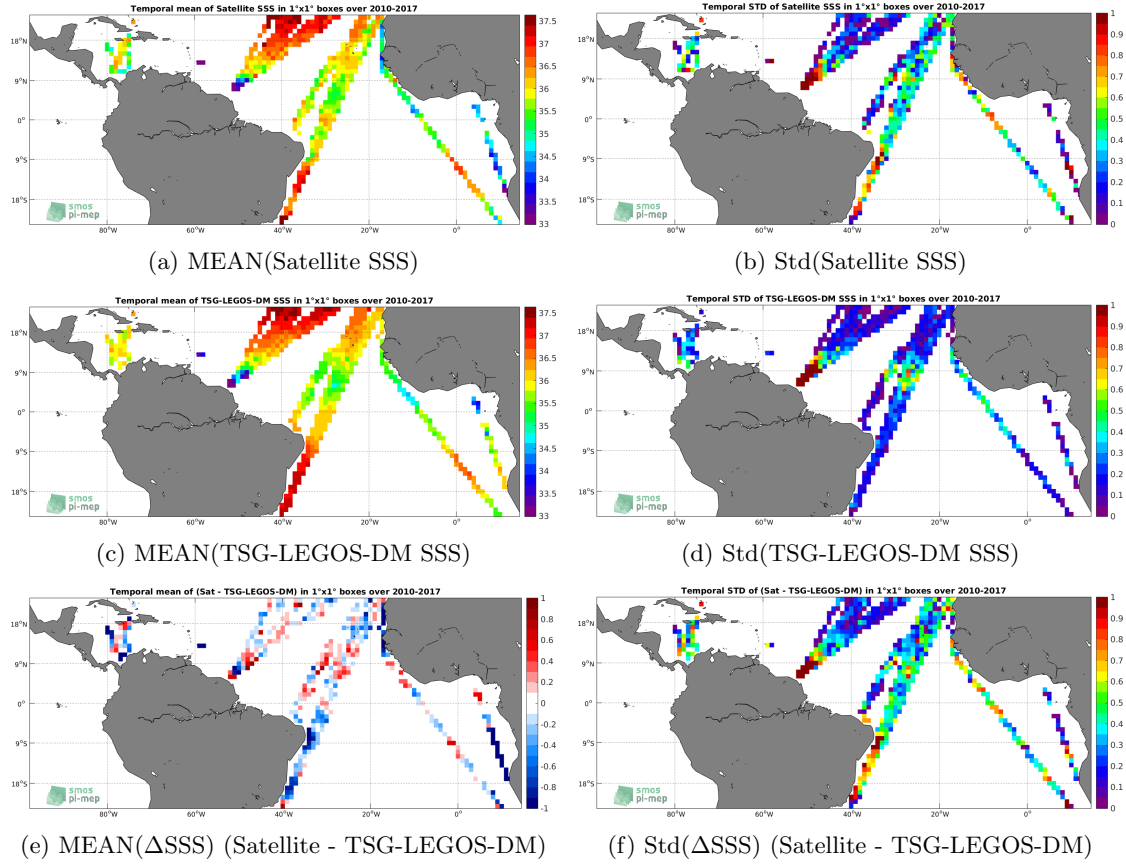
Figure 6: Temporal mean (left) and Std (right) of SSS from SMOS L3 v2 - Daily - 0.5 Deg (CATDS-CECOS-IFREMER) (top), TSG-LEGOS-DM (middle), and of \Delta SSS (Satellite - TSG-LEGOS-DM). Only match-up pairs are used to generate these maps.
