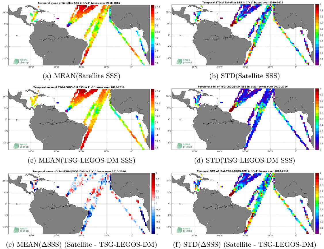
Figure 6: Temporal mean (left) and STD (right) of SSS from SMOS-L3-CATDS-CECOS-IFREMER-V2-1DAY-0.5DEG (top), TSG-LEGOS-DM (middle), and of \Delta SSS (Satellite - TSG-LEGOS-DM). Only match-up pairs are used to generate these maps.
