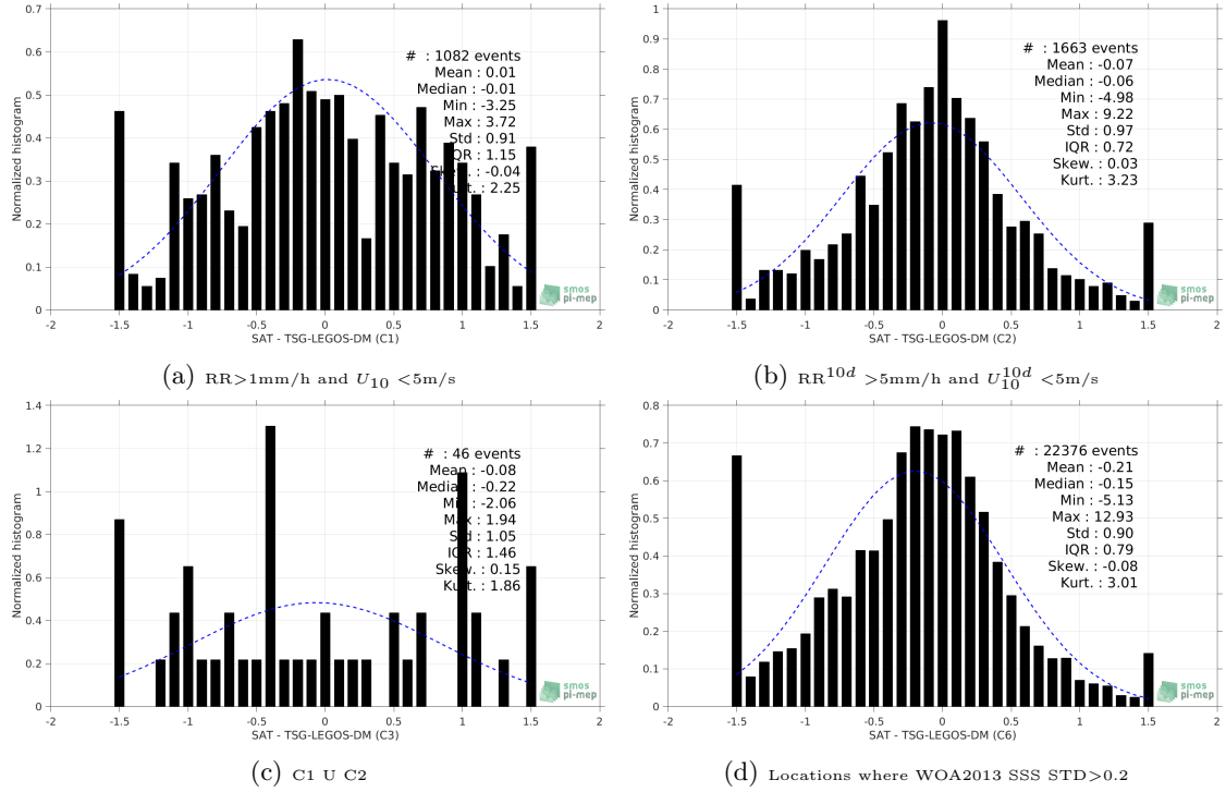
Figure 13: Normalized histogram of \Delta SSS (SMOS-L3-CATDS-CECOS-IFREMER-V2-1DAY-0.5DEG - TSG-LEGOS-DM) for 6 different subdatasets corresponding to: RR > 1mm/h and U_{10} < 5 m/s (a), RR^{10d} > 5 mm/h and U_{10}^{10d} < 5 m/s (b), C1 U C2 (c), Locations where WOA2013 SSS STD > 0.2 (d).
