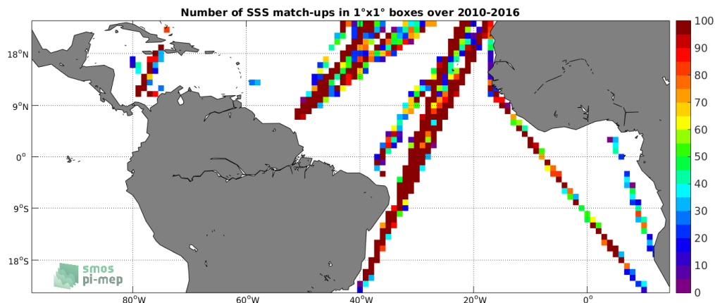
Figure 4: Number of SSS match-ups between TSG-LEGOS-DM SSS and the SMOS-L3-CATDS-CECOS-IFREMER-V2-1DAY-0.5DEG SSS product for the Tropical Atlantic Ocean Pi-MEP region over 1^\circ \times 1^\circ boxes and for the full satellite product period.
