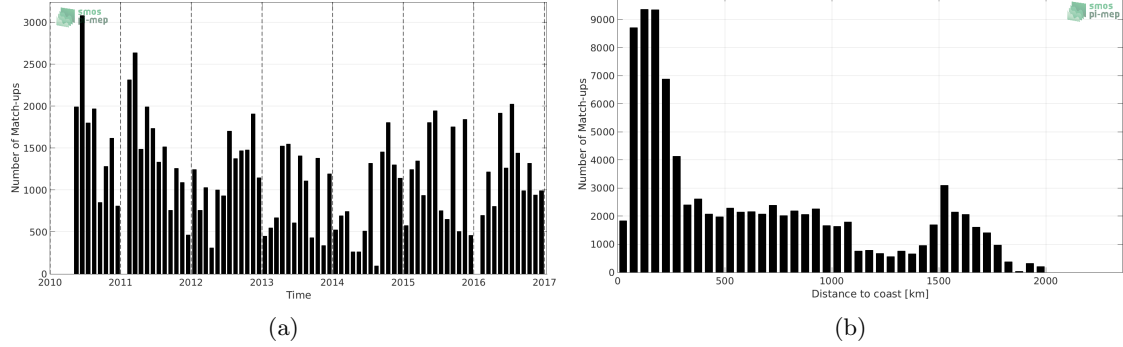
Figure 1: Number of match-ups between TSG-LEGOS-DM and SMOS-L3-CATDS-CECOS-IFREMER-V2-1DAY-0.5DEG SSS as a function of time (a) and as function of the distance to coast (b) over the Tropical Atlantic Ocean Pi-MEP region and for the full satellite product period.
