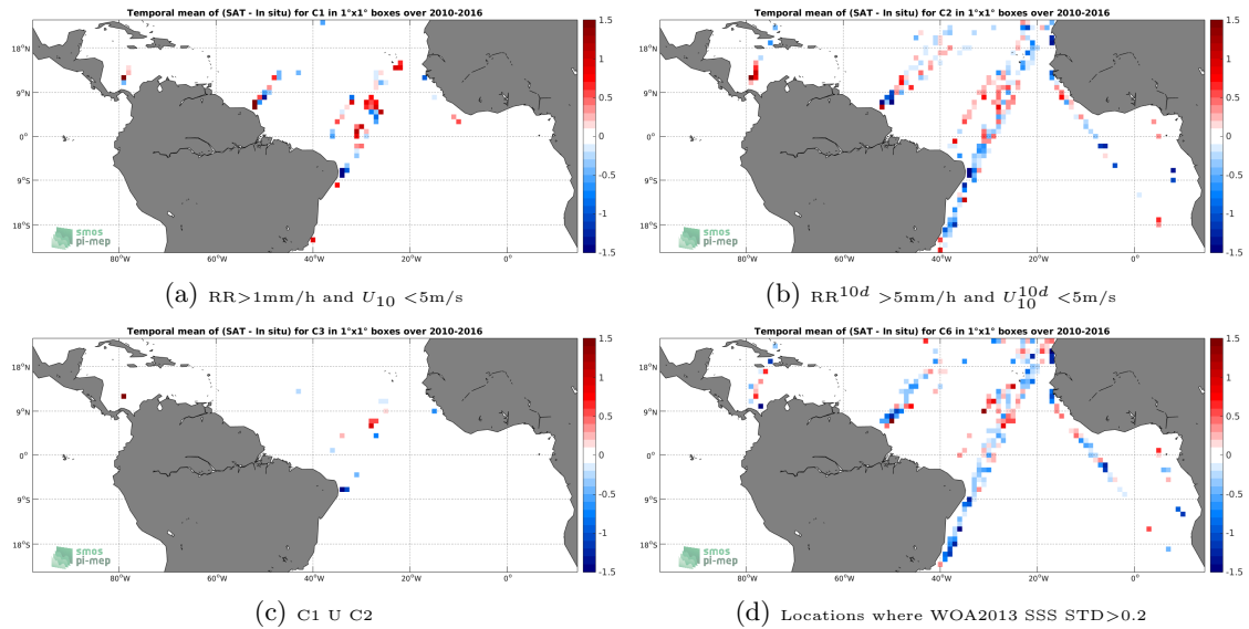
Figure 12: Temporal mean gridded over spatial boxes of size 1^\circ \times 1^\circ of \Delta SSS (SMOS-L3-CATDS-CECOS-IFREMER-V2-1DAY-0.5DEG - TSG-LEGOS-DM) for 4 different subdatasets corresponding to: RR > 1mm/h and U_{10} < 5\text{m/s} (a), RR^{10d} > 5\text{mm/h} and U_{10}^{10d} < 5\text{m/s} (b), C1 U C2 (c), Locations where WOA2013 SSS STD > 0.2 (d).
