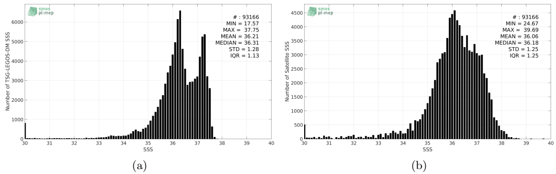
Figure 2: Histograms of SSS from TSG-LEGOS-DM (a) and SMOS-L3-CATDS-CECOS-IFREMER-V2-1DAY-0.5DEG (b) considering all match-up pairs per bins of 0.1 over the Tropical Atlantic Ocean Pi-MEP region and for the full satellite product period.
