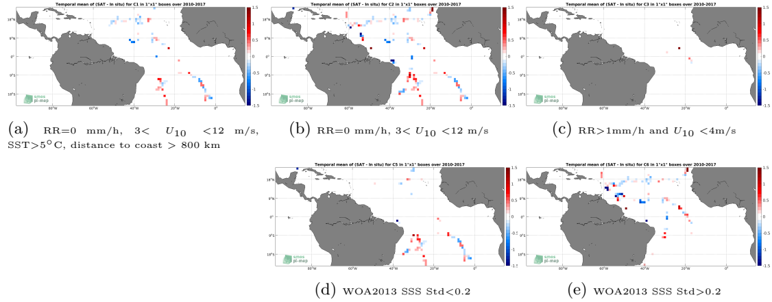
Figure 12: Temporal mean gridded over spatial boxes of size 1^{\circ}\times 1^{\circ} of \Delta SSS (SMOS SSS L3 v2 - Daily - 0.5 Deg (CATDS-CECOS-IFREMER) - TSG (GOSUD-Sailing-ship)) for 5 different subdatasets corresponding to:RR=0 mm/h, 3 < U_{10} < 12 m/s, SST >5^{\circ}\text{C} , distance to coast > 800 km (a), RR=0 mm/h, 3 < U_{10} < 12 m/s (b), RR >1 mm/h and U_{10} < 4 m/s (c), WOA2013 SSS Std <0.2 (d), WOA2013 SSS Std >0.2 (e).
