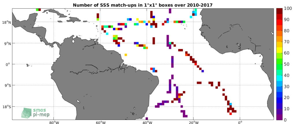
Figure 4: Number of SSS match-ups between TSG (GOSUD-Sailing-ship) SSS and the SMOS SSS L3 v2 - Daily - 0.5 Deg (CATDS-CECOS-IFREMER) SSS product for the Tropical Atlantic Ocean Pi-MEP region over 1^\circ \times 1^\circ boxes and for the full satellite product period.
