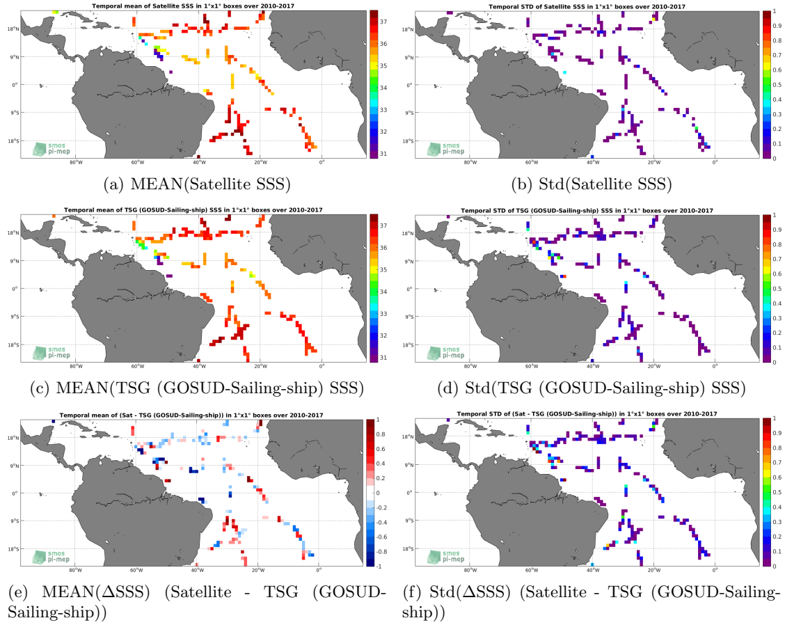
Figure 6: Temporal mean (left) and Std (right) of SSS from SMOS SSS L3 v2 - Daily - 0.5 Deg (CATDS-CECOS-IFREMER) (top), TSG (GOSUD-Sailing-ship) (middle), and of \Delta SSS (Satellite - TSG (GOSUD-Sailing-ship)). Only match-up pairs are used to generate these maps.
