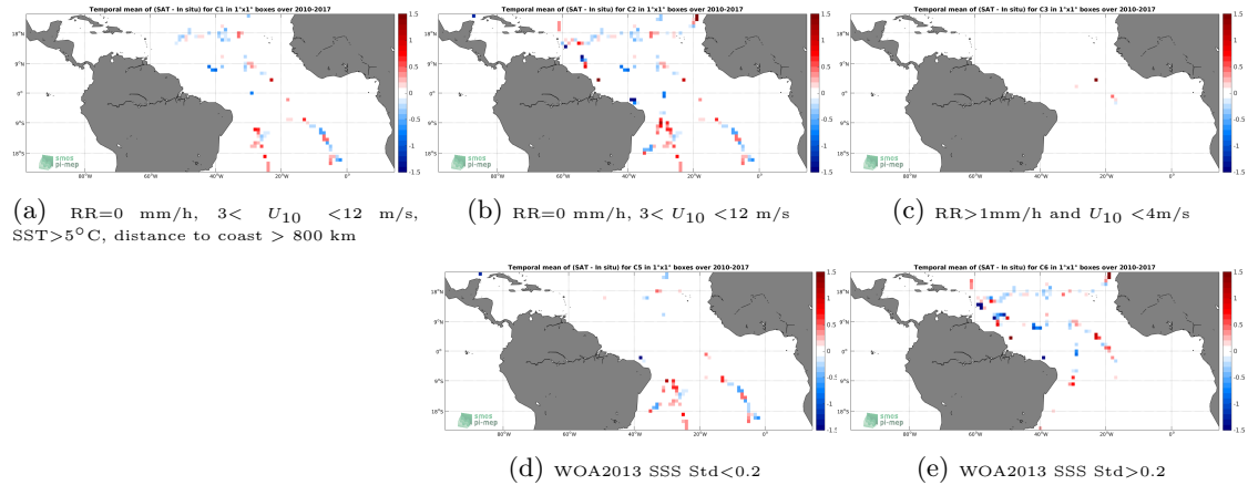
Figure 12: Temporal mean gridded over spatial boxes of size 1^\circ \times 1^\circ of \Delta SSS (SMOS SSS L3 v2 - Daily - 0.5 Deg (CATDS-CECOS-IFREMER) - TSG (GOSUD-Sailing-ship)) for 5 different subdatasets corresponding to:RR=0 mm/h, 3 < U_{10} < 12 m/s, SST >5^\circ\text{C} , distance to coast > 800 km (a), RR=0 mm/h, 3 < U_{10} < 12 m/s (b), RR >1 mm/h and U_{10} < 4 m/s (c), WOA2013 SSS Std <0.2 (d), WOA2013 SSS Std >0.2 (e).
