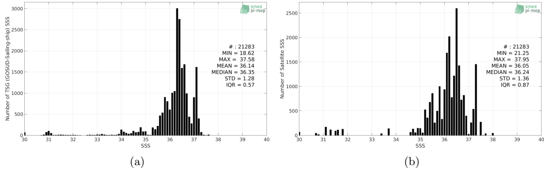
Figure 2: Histograms of SSS from TSG (GOSUD-Sailing-ship) (a) and SMOS SSS L3 v2 - Daily - 0.5 Deg (CATDS-CECOS-IFREMER) (b) considering all match-up pairs per bins of 0.1 over the Tropical Atlantic Ocean Pi-MEP region and for the full satellite product period.
