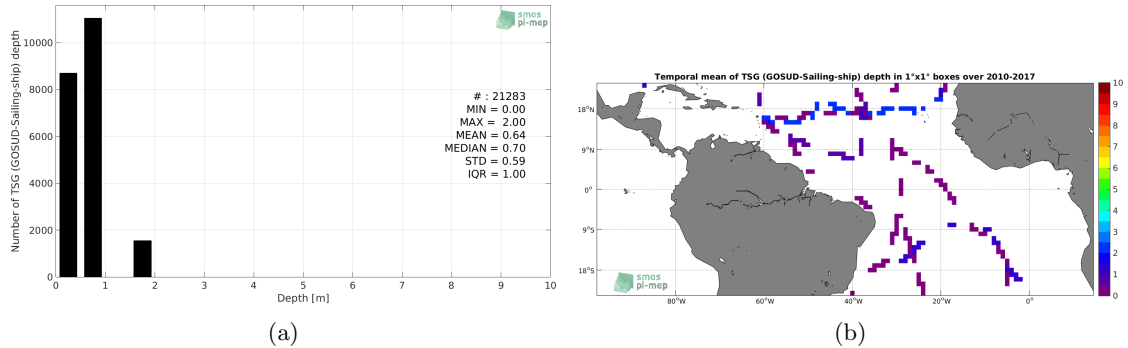
Figure 3: Histograms of the depth of the upper level SSS measurements from TSG (GOSUD-Sailing-ship) in the Match-up DataBase for the Tropical Atlantic Ocean Pi-MEP region (a) and temporal mean spatial distribution of pressure of the in situ SSS data over 1^\circ \times 1^\circ boxes and for the full satellite product period (b).
