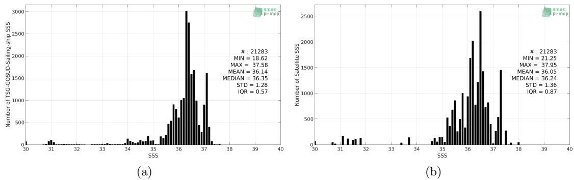
Figure 2: Histograms of SSS from TSG-GOSUD-Sailing-ship (a) and SMOS L3 v2 - Daily - 0.5 Deg (CATDS-CECOS-IFREMER) (b) considering all match-up pairs per bins of 0.1 over the Tropical Atlantic Ocean Pi-MEP region and for the full satellite product period.
