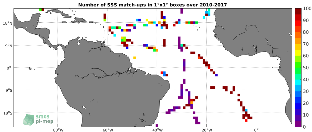
Figure 4: Number of SSS match-ups between TSG-GOSUD-Sailing-ship SSS and the SMOS L3 v2 - Daily - 0.5 Deg (CATDS-CECOS-IFREMER) SSS product for the Tropical Atlantic Ocean Pi-MEP region over 1^\circ \times 1^\circ boxes and for the full satellite product period.
