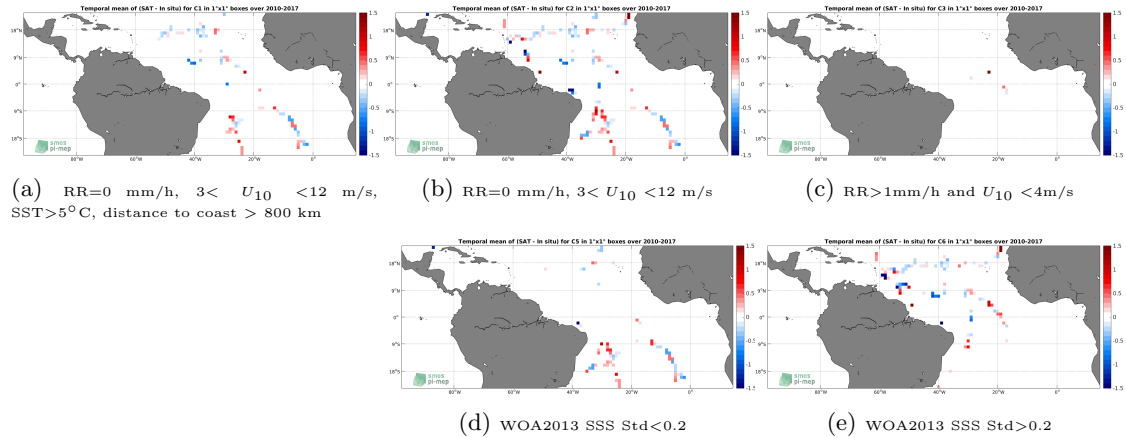
Figure 12: Temporal mean gridded over spatial boxes of size 1^{\circ}\times 1^{\circ} of \Delta SSS (SMOS L3 v2 - Daily - 0.5 Deg (CATDS-CECOS-IFREMER) - TSG-GOSUD-Sailing-ship) for 5 different subdatasets corresponding to:RR=0 mm/h, 3 < U_{10} < 12 m/s, SST >5^{\circ}\text{C} , distance to coast > 800 km (a), RR=0 mm/h, 3 < U_{10} < 12 m/s (b), RR >1 mm/h and U_{10} < 4 m/s (c), WOA2013 SSS Std <0.2 (d), WOA2013 SSS Std >0.2 (e).
