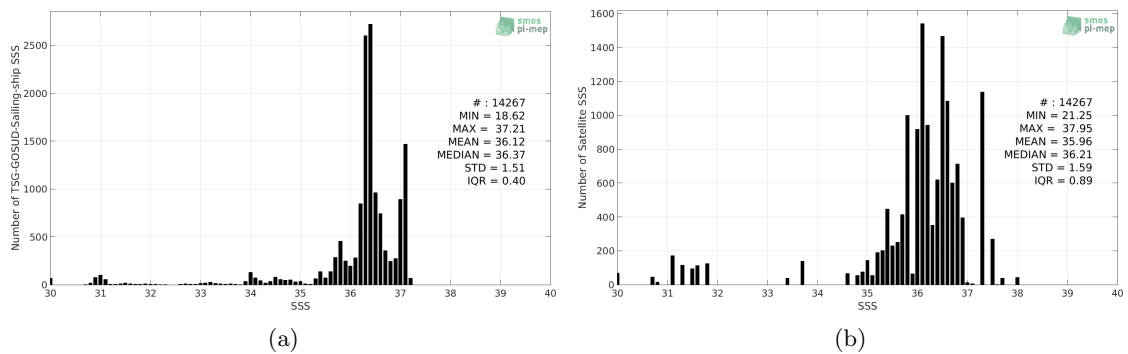
Figure 2: Histograms of SSS from TSG-GOSUD-Sailing-ship (a) and SMOS-L3-CATDS-CECOS-IFREMER-V2-1DAY-0.5DEG (b) considering all match-up pairs per bins of 0.1 over the Tropical Atlantic Ocean Pi-MEP region and for the full satellite product period.
