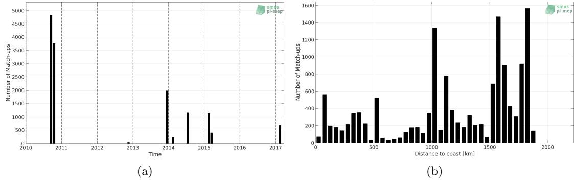
Figure 1: Number of match-ups between TSG-GOSUD-Sailing-ship and SMOS-L3-CATDS-CECOS-IFREMER-V2-1DAY-0.5DEG SSS as a function of time (a) and as function of the distance to coast (b) over the Tropical Atlantic Ocean Pi-MEP region and for the full satellite product period.
