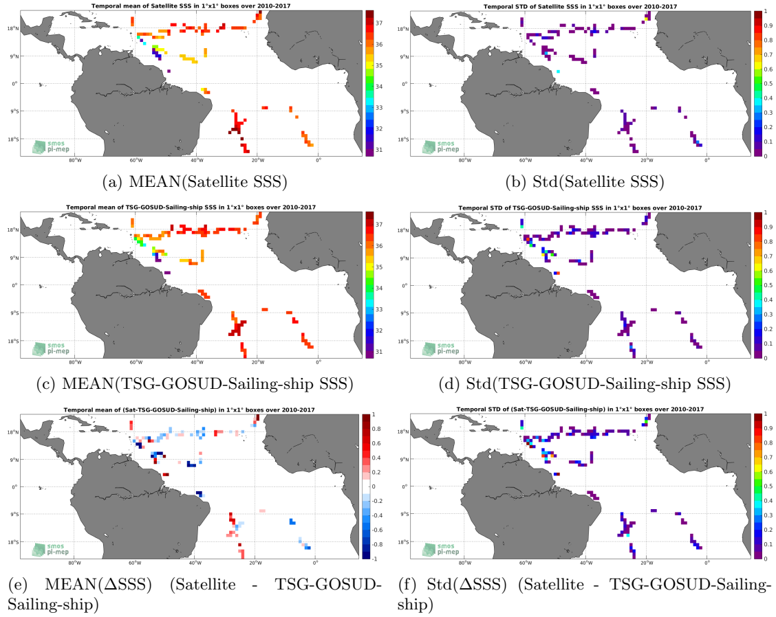
Figure 6: Temporal mean (left) and Std (right) of SSS from SMOS-L3-CATDS-CECOS-IFREMER-V2-1DAY-0.5DEG (top), TSG-GOSUD-Sailing-ship (middle), and of \Delta SSS (Satellite - TSG-GOSUD-Sailing-ship). Only match-up pairs are used to generate these maps.
