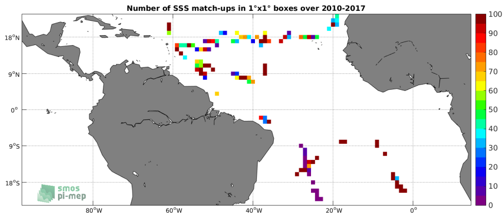
Figure 4: Number of SSS match-ups between TSG-GOSUD-Sailing-ship SSS and the SMOS-L3-CATDS-CECOS-IFREMER-V2-1DAY-0.5DEG SSS product for the Tropical Atlantic Ocean Pi-MEP region over 1^\circ \times 1^\circ boxes and for the full satellite product period.
