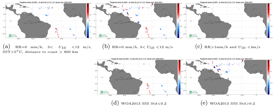
Figure 12: Temporal mean gridded over spatial boxes of size 1^\circ \times 1^\circ of \Delta SSS (SMOS-L3-CATDS-CECOS-IFREMER-V2-1DAY-0.5DEG - TSG-GOSUD-Sailing-ship) for 5 different subdatasets corresponding to:RR=0 mm/h, 3 < U_{10} < 12 m/s, SST >5^\circ C, distance to coast > 800 km (a), RR=0 mm/h, 3 < U_{10} < 12 m/s (b), RR >1 mm/h and U_{10} < 4 m/s (c), WOA2013 SSS Std <0.2 (d), WOA2013 SSS Std >0.2 (e).
