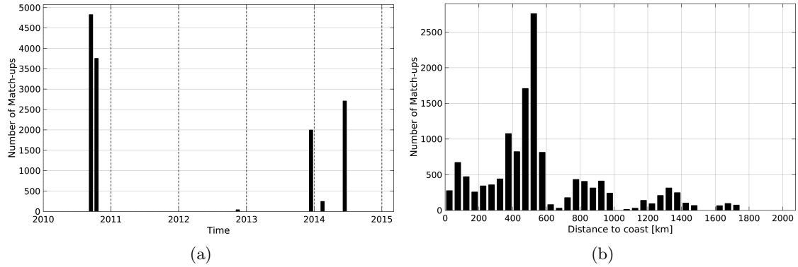
Figure 1: Number of match-ups between TSG-GOSUD-Sailing-ship and SMOS-L3-CATDS-CECOS-IFREMER-V2-1DAY-0.5deg SSS as a function of time (a) and as function of the distance to coast (b) over the Tropical Atlantic Ocean Pi-MEP region and for the full satellite product period.
