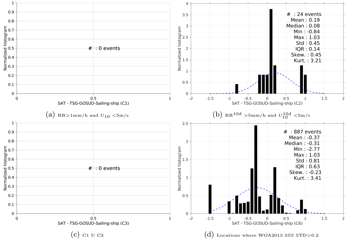
Figure 13: Normalized histogram of \Delta SSS (SMOS-L3-CATDS-CECOS-IFREMER-V2-1DAY-0.5deg - TSG-GOSUD-Sailing-ship) for 6 different subdatasets corresponding to: RR > 1\text{mm/h} and U_{10} < 5\text{m/s} (a), RR^{10d} > 5\text{mm/h} and U_{10}^{10d} < 5\text{m/s} (b), C1 \cup C2 (c), Locations where WOA2013 SSS STD > 0.2 (d).
