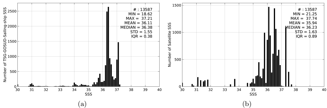
Figure 2: Histograms of SSS from TSG-GOSUD-Sailing-ship (a) and SMOS-L3-CATDS-CECOS-IFREMER-V2-1DAY-0.5deg (b) considering all match-up pairs per bins of 0.1 over the Tropical Atlantic Ocean Pi-MEP region and for the full satellite product period.
