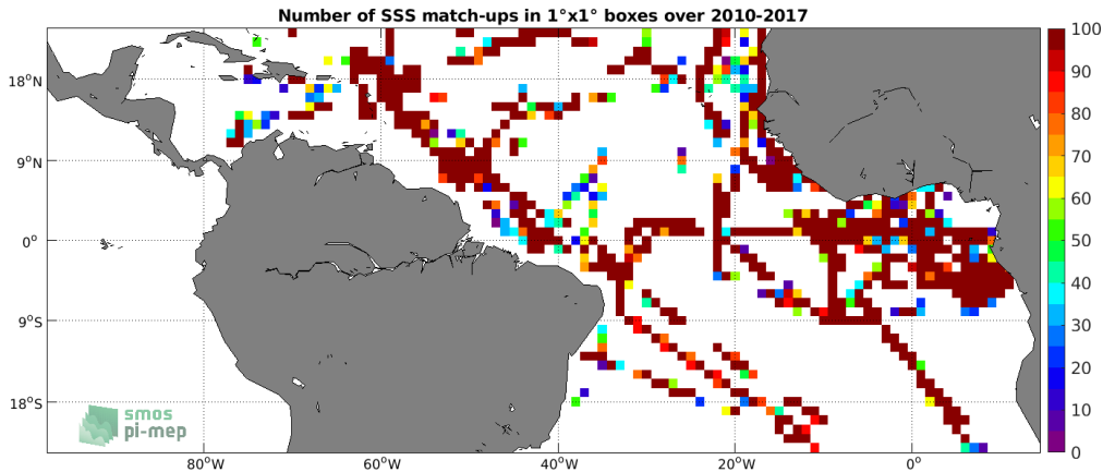
Figure 4: Number of SSS match-ups between TSG (GOSUD-Research-vessel) SSS and the SMOS SSS L3 v2 - Daily - 0.5 Deg (CATDS-CECOS-IFREMER) SSS product for the Tropical Atlantic Ocean Pi-MEP region over 1°x1° boxes and for the full satellite product period.
