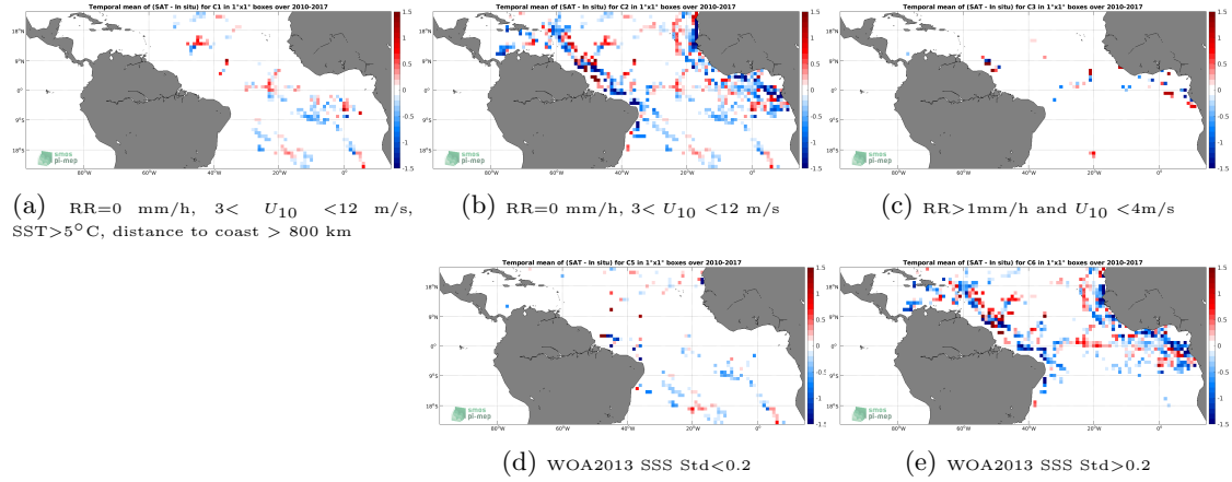
Figure 12: Temporal mean gridded over spatial boxes of size 1^{\circ}\times 1^{\circ} of \Delta SSS (SMOS SSS L3 v2 - Daily - 0.5 Deg (CATDS-CECOS-IFREMER) - TSG (GOSUD-Research-vessel)) for 5 different subdatasets corresponding to:RR=0 mm/h, 3 < U_{10} < 12 m/s, SST >5^{\circ}\text{C} , distance to coast > 800 km (a), RR=0 mm/h, 3 < U_{10} < 12 m/s (b), RR >1 mm/h and U_{10} < 4 m/s (c), WOA2013 SSS Std <0.2 (d), WOA2013 SSS Std >0.2 (e).
