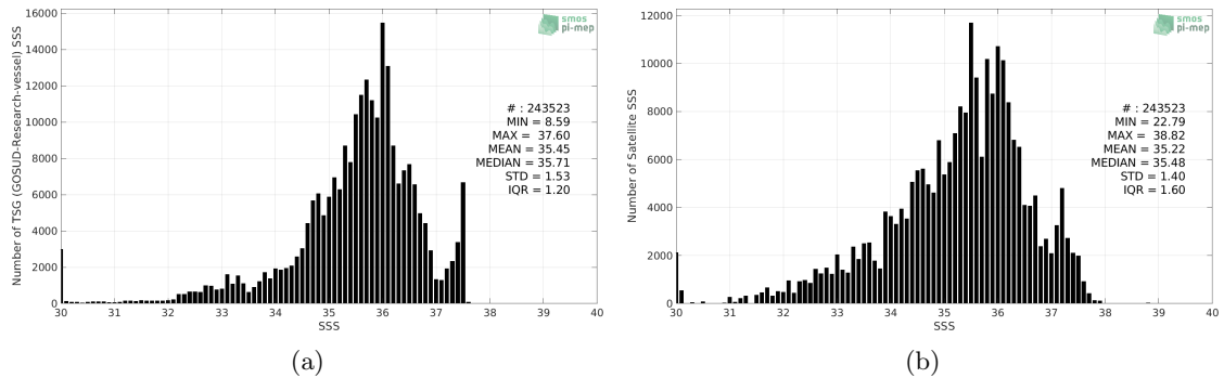
Figure 2: Histograms of SSS from TSG (GOSUD-Research-vessel) (a) and SMOS SSS L3 v2 - Daily - 0.5 Deg (CATDS-CECOS-IFREMER) (b) considering all match-up pairs per bins of 0.1 over the Tropical Atlantic Ocean Pi-MEP region and for the full satellite product period.
