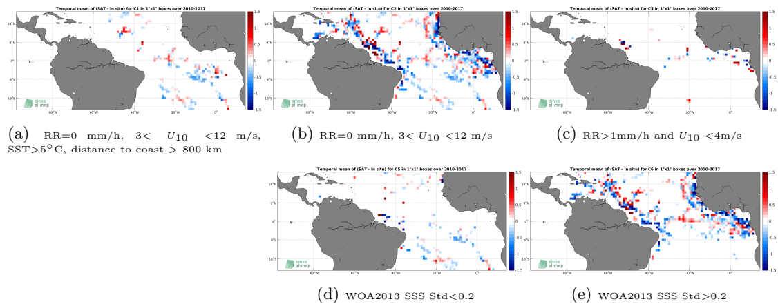
Figure 12: Temporal mean gridded over spatial boxes of size 1^\circ \times 1^\circ of \Delta SSS (SMOS-L3-CATDS-CECOS-IFREMER-V2-1DAY-0.5DEG - TSG-GOSUD-Research-vessel) for 5 different subdatasets corresponding to:RR=0 mm/h, 3 < U_{10} < 12 m/s, SST > 5^\circ\text{C} , distance to coast > 800 km (a), RR=0 mm/h, 3 < U_{10} < 12 m/s (b), RR > 1 mm/h and U_{10} < 4 m/s (c), WOA2013 SSS Std < 0.2 (d), WOA2013 SSS Std > 0.2 (e).
