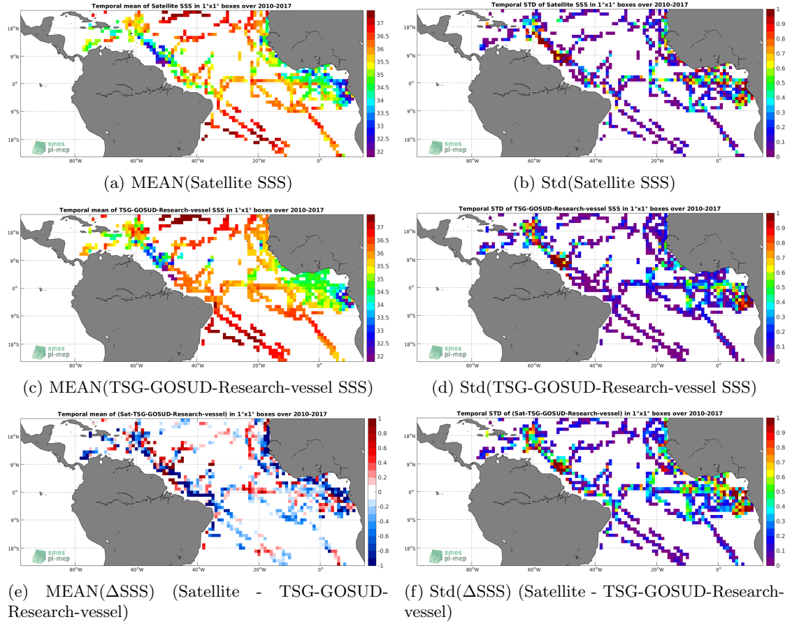
Figure 6: Temporal mean (left) and Std (right) of SSS from SMOS-L3-CATDS-CECOS-IFREMER-V2-1DAY-0.5DEG (top), TSG-GOSUD-Research-vessel (middle), and of \Delta SSS (Satellite - TSG-GOSUD-Research-vessel). Only match-up pairs are used to generate these maps.
