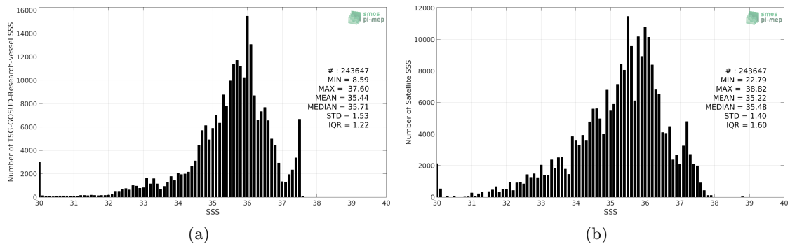
Figure 2: Histograms of SSS from TSG-GOSUD-Research-vessel (a) and SMOS-L3-CATDS-CECOS-IFREMER-V2-1DAY-0.5DEG (b) considering all match-up pairs per bins of 0.1 over the Tropical Atlantic Ocean Pi-MEP region and for the full satellite product period.
