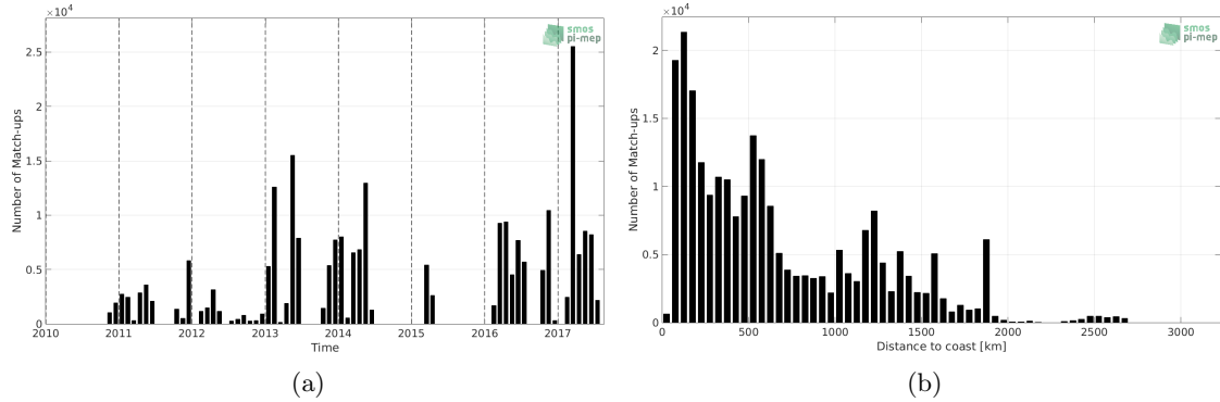
Figure 1: Number of match-ups between TSG-GOSUD-Research-vessel and SMOS-L3-CATDS-CECOS-IFREMER-V2-1DAY-0.5DEG SSS as a function of time (a) and as function of the distance to coast (b) over the Tropical Atlantic Ocean Pi-MEP region and for the full satellite product period.
