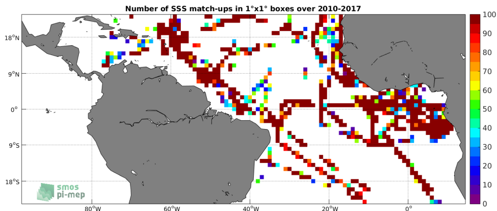
Figure 4: Number of SSS match-ups between TSG-GOSUD-Research-vessel SSS and the SMOS-L3-CATDS-CECOS-IFREMER-V2-1DAY-0.5DEG SSS product for the Tropical Atlantic Ocean Pi-MEP region over 1^\circ \times 1^\circ boxes and for the full satellite product period.
