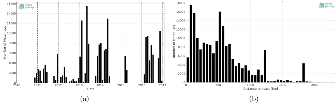
Figure 1: Number of match-ups between TSG-GOSUD-Research-vessel and SMOS-L3-CATDS-CECOS-IFREMER-V2-1DAY-0.5DEG SSS as a function of time (a) and as function of the distance to coast (b) over the Tropical Atlantic Ocean Pi-MEP region and for the full satellite product period.
