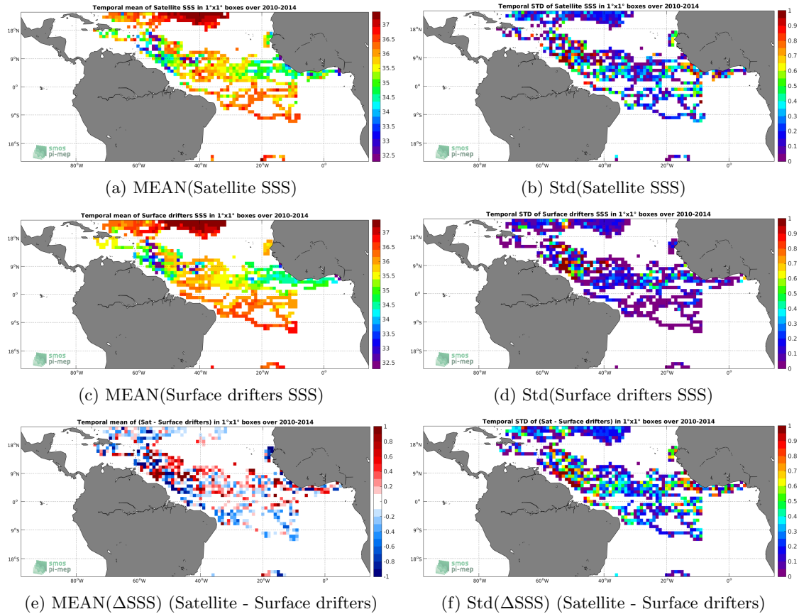
Figure 5: Temporal mean (left) and Std (right) of SSS from SMOS L3 v2 - Daily - 0.5 Deg (CATDS-CECOS-IFREMER) (top), Surface drifters (middle), and of \Delta SSS (Satellite - Surface drifters). Only match-up pairs are used to generate these maps.
