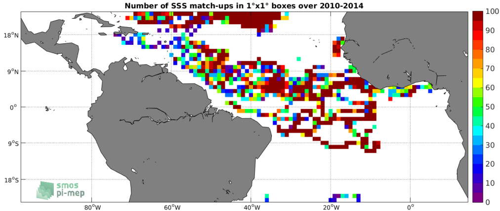
Figure 3: Number of SSS match-ups between Surface drifters SSS and the SMOS L3 v2 - Daily - 0.5 Deg (CATDS-CECOS-IFREMER) SSS product for the Tropical Atlantic Ocean Pi-MEP region over 1°x1° boxes and for the full satellite product period.
