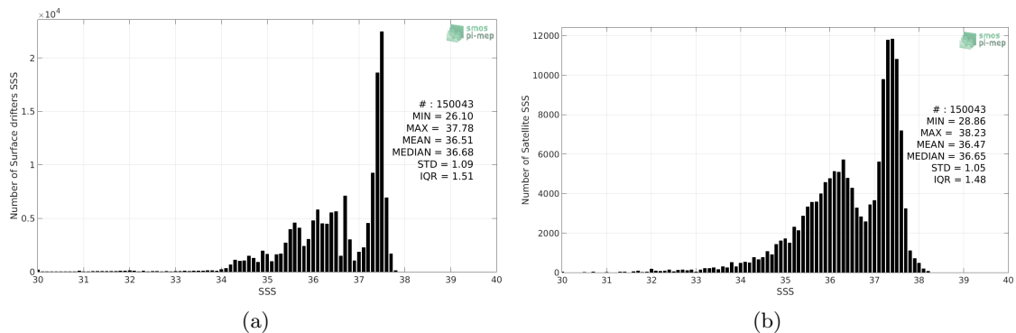
Figure 2: Histograms of SSS from Surface drifters (a) and SMOS L3 v2 - Daily - 0.5 Deg (CATDS-CECOS-IFREMER) (b) considering all match-up pairs per bins of 0.1 over the Tropical Atlantic Ocean Pi-MEP region and for the full satellite product period.
