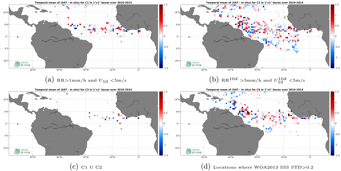
Figure 11: Temporal mean gridded over spatial boxes of size 1^\circ \times 1^\circ of \Delta\text{SSS} (SMOS-L3-CATDS-CECOS-IFREMER-V2-1DAY-0.5DEG - Surface drifters) for 4 different subdatasets corresponding to: RR > 1\text{mm/h} and U_{10} < 5\text{m/s} (a), RR^{10d} > 5\text{mm/h} and U_{10}^{10d} < 5\text{m/s} (b), C1 U C2 (c), Locations where WOA2013 SSS STD > 0.2 (d).
