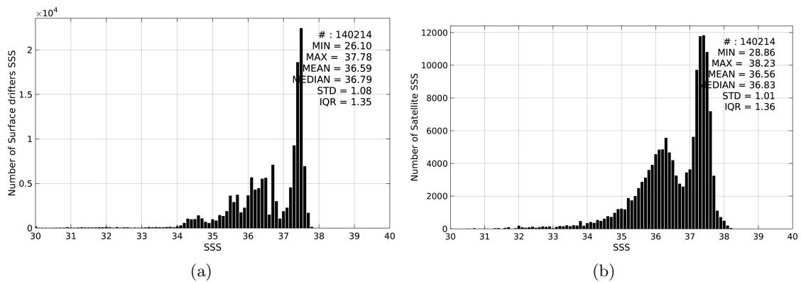
Figure 2: Histograms of SSS from Surface drifters (a) and SMOS-L3-CATDS-CECOS-IFREMER-V2-1DAY-0.5deg (b) considering all match-up pairs per bins of 0.1 over the Tropical Atlantic Ocean Pi-MEP region and for the full satellite product period.
