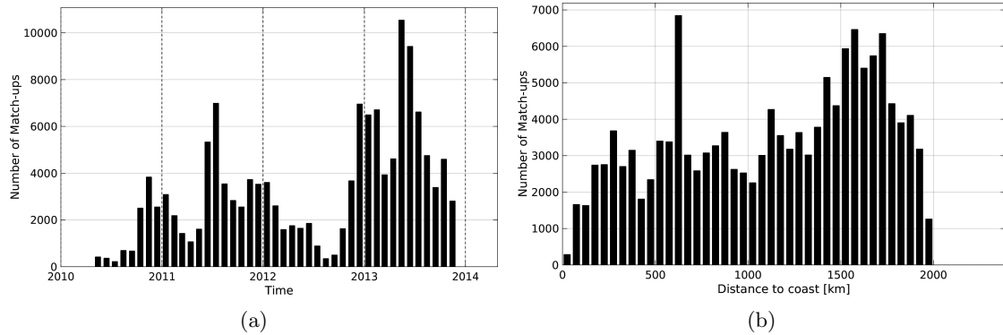
Figure 1: Number of match-ups between Surface drifters and SMOS-L3-CATDS-CECOS-IFREMER-V2-1DAY-0.5deg SSS as a function of time (a) and as function of the distance to coast (b) over the Tropical Atlantic Ocean Pi-MEP region and for the full satellite product period.
