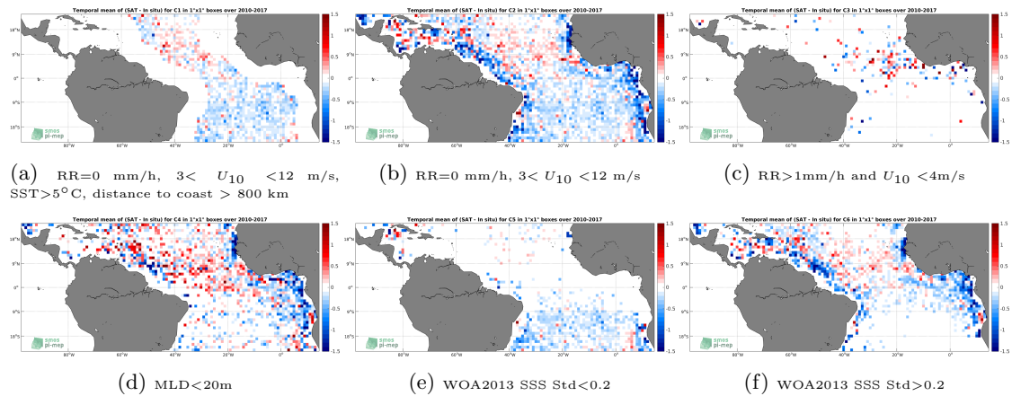
Figure 12: Temporal mean gridded over spatial boxes of size 1^\circ \times 1^\circ of \Delta SSS (SMOS-L3-CATDS-CECOS-IFREMER-V2-1DAY-0.5DEG - Argo) for 6 different subdatasets corresponding to:RR=0 mm/h, 3 < U_{10} < 12 m/s, SST >5^\circ C, distance to coast > 800 km (a), RR=0 mm/h, 3 < U_{10} < 12 m/s (b), RR >1 mm/h and U_{10} < 4 m/s (c),MLD <20 m (d),WOA2013 SSS Std <0.2 (e),WOA2013 SSS Std >0.2 (f).
