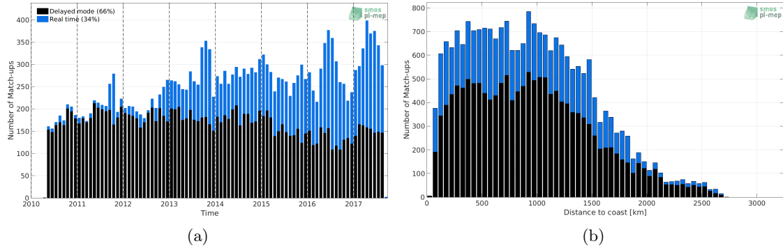
Figure 1: Number of match-ups between Argo and SMOS-L3-CATDS-CECOS-IFREMER-V2-1DAY-0.5DEG SSS as a function of time (a) and as function of the distance to coast (b) over the Tropical Atlantic Ocean Pi-MEP region and for the full satellite product period.
