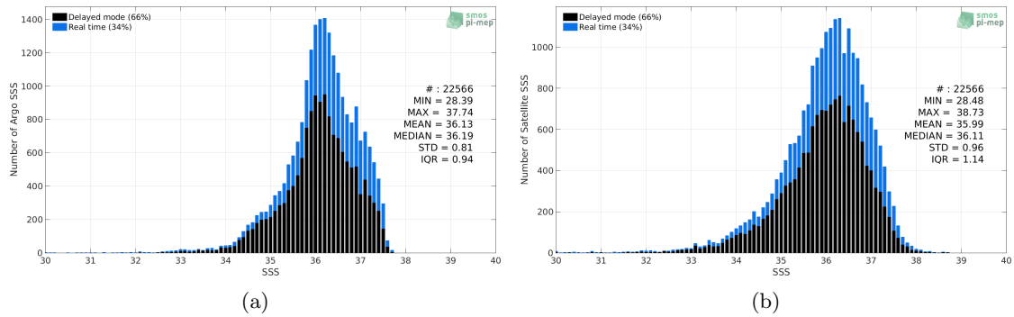
Figure 2: Histograms of SSS from Argo (a) and SMOS-L3-CATDS-CECOS-IFREMER-V2-1DAY-0.5DEG (b) considering all match-up pairs per bins of 0.1 over the Tropical Atlantic Ocean Pi-MEP region and for the full satellite product period.
