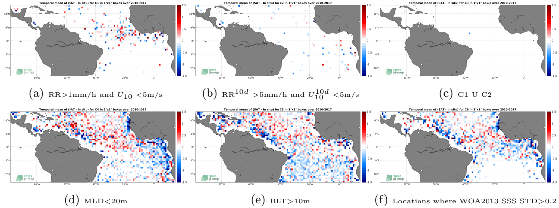
Figure 12: Temporal mean gridded over spatial boxes of size 1^\circ \times 1^\circ of \Delta\text{SSS} (SMOS-L3-CATDS-CECOS-IFREMER-V2-1DAY-0.5DEG - Argo) for 6 different subdatasets corresponding to: \text{RR} > 1\text{mm/h} and U_{10} < 5\text{m/s} (a), \text{RR}^{10d} > 5\text{mm/h} and U_{10}^{10d} < 5\text{m/s} (b), C1 U C2 (c), \text{MLD} < 20\text{m} (d), \text{BLT} > 10\text{m} (e), Locations where WOA2013 SSS \text{STD} > 0.2 (f).
