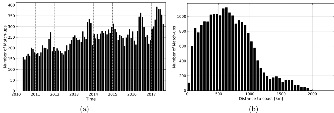
Figure 1: Number of match-ups between Argo and SMOS-L3-CATDS-CECOS-IFREMER-V2-1DAY-0.5DEG SSS as a function of time (a) and as function of the distance to coast (b) over the Tropical Atlantic Ocean Pi-MEP region and for the full satellite product period.
