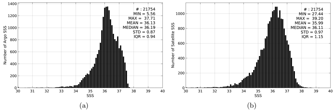
Figure 2: Histograms of SSS from Argo (a) and SMOS-L3-CATDS-CECOS-IFREMER-V2-1DAY-0.5deg (b) considering all match-up pairs per bins of 0.1 over the Tropical Atlantic Ocean Pi-MEP region and for the full satellite product period.
