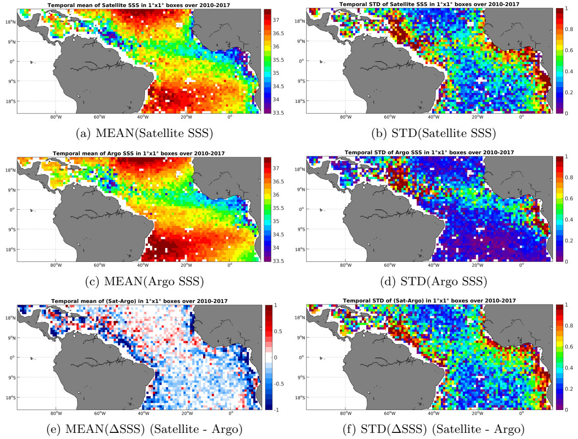
Figure 6: Temporal mean (left) and STD (right) of SSS from SMOS-L3-CATDS-CECOS-IFREMER-V2-1DAY-0.5deg (top), Argo (middle), and of \Delta SSS (Satellite - Argo). Only match-up pairs are used to generate these maps.
