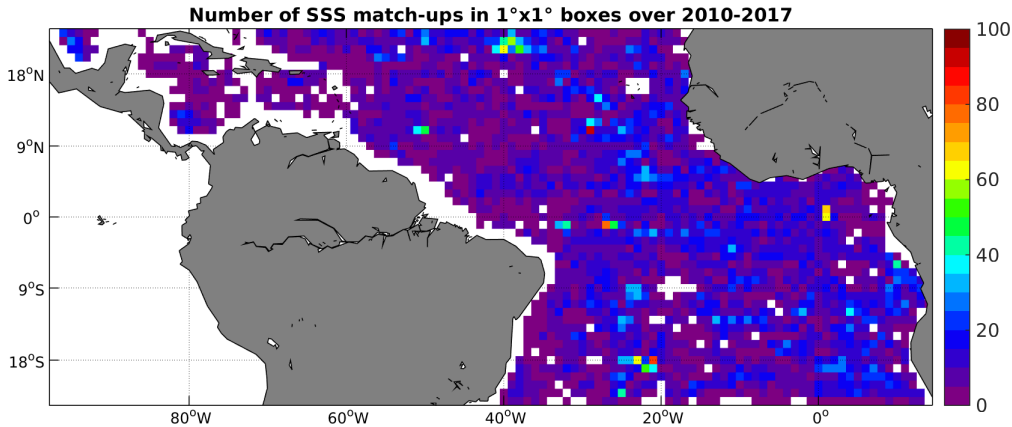
Figure 4: Number of SSS match-ups between Argo SSS and the SMOS-L3-CATDS-CECOS-IFREMER-V2-1DAY-0.5deg SSS product for the Tropical Atlantic Ocean Pi-MEP region over 1^\circ \times 1^\circ boxes and for the full satellite product period.
