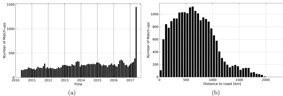
Figure 1: Number of match-ups between Argo and SMOS-L3-CATDS-CECOS-IFREMER-V2-1DAY-0.5deg SSS as a function of time (a) and as function of the distance to coast (b) over the Tropical Atlantic Ocean Pi-MEP region and for the full satellite product period.
