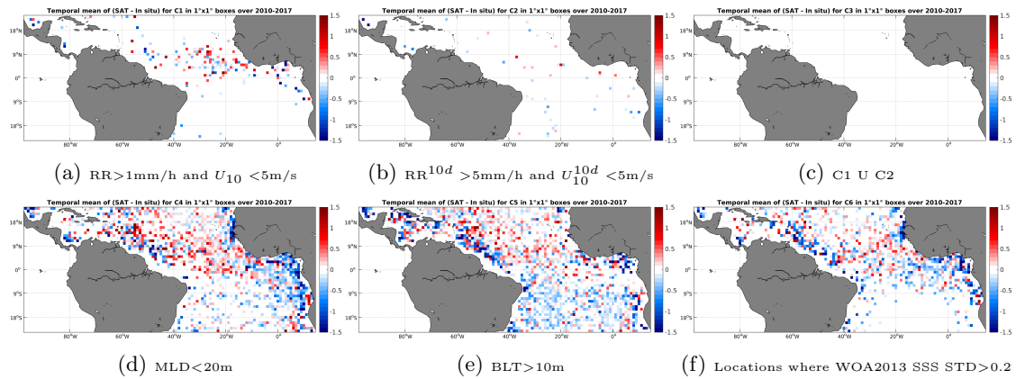
Figure 12: Temporal mean gridded over spatial boxes of size 1^\circ \times 1^\circ of \Delta SSS (SMOS-L3-CATDS-CECOS-IFREMER-V2-1DAY-0.5deg - Argo) for 6 different subdatasets corresponding to: RR > 1mm/h and U_{10} < 5\text{m/s} (a), RR^{10d} > 5\text{mm/h} and U_{10}^{10d} < 5\text{m/s} (b), C1 U C2 (c), MLD < 20m (d), BLT > 10m (e), Locations where WOA2013 SSS STD > 0.2 (f).
