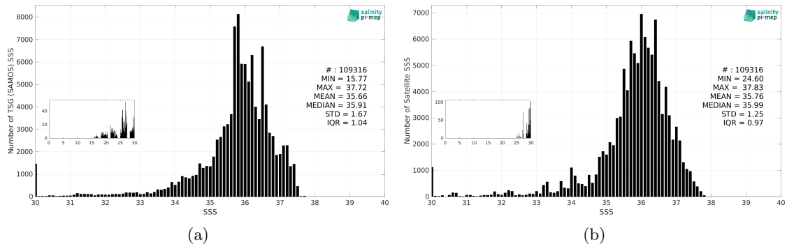
Figure 3: Histograms of SSS from TSG (SAMOS) (a) and SMOS SSS L3 v335 - Monthly - 25 km (CATDS-CPDC) (b) considering all match-up pairs per bins of 0.1 over the Tropical Atlantic Ocean Pi-MEP region and for the full satellite product period.
