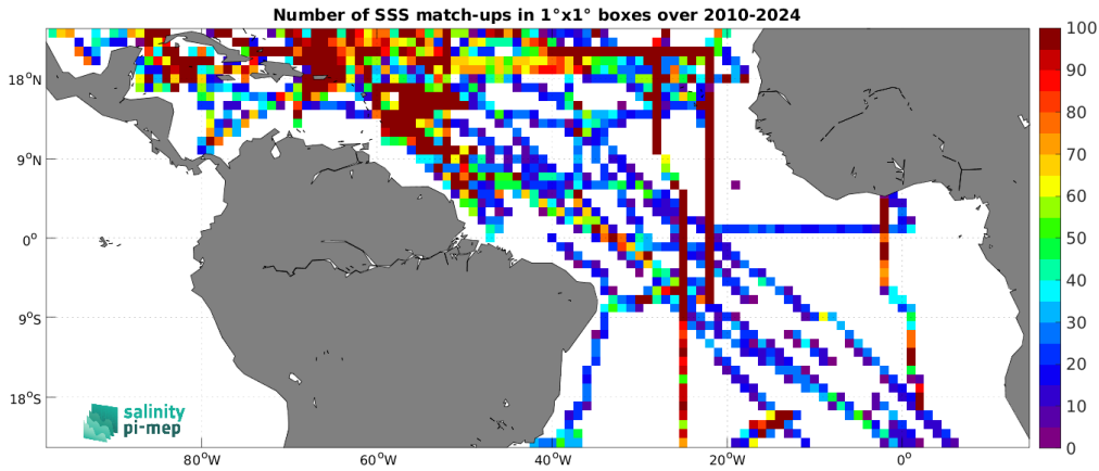
Figure 5: Number of SSS match-ups between TSG (SAMOS) SSS and the SMOS SSS L3 v335 - Monthly - 25 km (CATDS-CPDC) SSS product for the Tropical Atlantic Ocean Pi-MEP region over 1^\circ \times 1^\circ boxes and for the full satellite product period.
