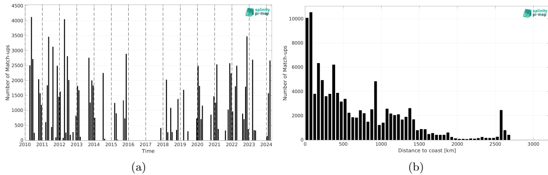
Figure 2: Number of match-ups between TSG (SAMOS) and SMOS SSS L3 v335 - Monthly - 25 km (CATDS-CPDC) SSS as a function of time (a) and as function of the distance to coast (b) over the Tropical Atlantic Ocean Pi-MEP region and for the full satellite product period.
