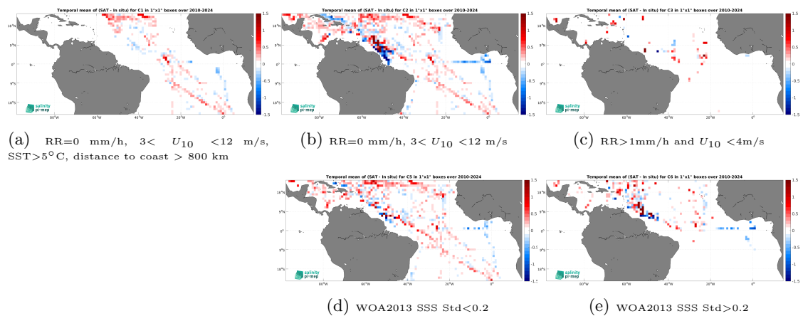
Figure 14: Temporal mean gridded over spatial boxes of size 1^\circ \times 1^\circ of \Delta\text{SSS} (SMOS SSS L3 v335 - Monthly - 25 km (CATDS-CPDC) - TSG (SAMOS)) for 5 different subdatasets corresponding to:RR=0 mm/h, 3 < U_{10} < 12 m/s, SST>5°C, distance to coast > 800 km (a), RR=0 mm/h, 3 < U_{10} < 12 m/s (b), RR>1mm/h and U_{10} < 4 m/s (c), WOA2013 SSS Std<0.2 (d), WOA2013 SSS Std>0.2 (e).
