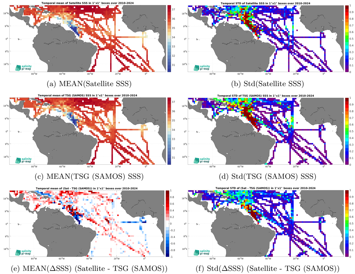
Figure 7: Temporal mean (left) and Std (right) of SSS from SMOS SSS L3 v335 - Monthly - 25 km (CATDS-CPDC) (top), TSG (SAMOS) (middle), and of \Delta\text{SSS} (Satellite - TSG (SAMOS)). Only match-up pairs are used to generate these maps.
