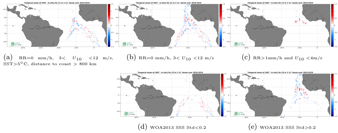
Figure 12: Temporal mean gridded over spatial boxes of size 1^\circ \times 1^\circ of \Delta SSS (SMOS SSS L3 v335 - Monthly - 25 km (CATDS-CPDC) - TSG (Polarstern)) for 5 different subdatasets corresponding to:RR=0 mm/h, 3 < U_{10} < 12 m/s, SST>5°C, distance to coast > 800 km (a), RR=0 mm/h, 3 < U_{10} < 12 m/s (b), RR>1mm/h and U_{10} < 4 m/s (c), WOA2013 SSS Std<0.2 (d), WOA2013 SSS Std>0.2 (e).
