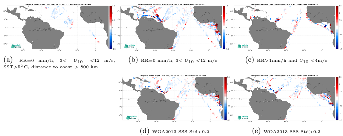
Figure 14: Temporal mean gridded over spatial boxes of size 1^\circ \times 1^\circ of \Delta\text{SSS} (SMOS SSS L3 v335 - Monthly - 25 km (CATDS-CPDC) - TSG (LEGOS-DM)) for 5 different subdatasets corresponding to:RR=0 mm/h, 3 < U_{10} < 12 m/s, SST >5^\circ\text{C} , distance to coast > 800 km (a), RR=0 mm/h, 3 < U_{10} < 12 m/s (b), RR >1 mm/h and U_{10} < 4 m/s (c), WOA2013 SSS Std <0.2 (d), WOA2013 SSS Std >0.2 (e).
