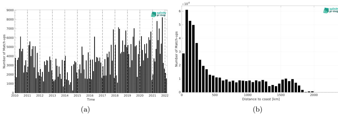
Figure 2: Number of match-ups between TSG (LEGOS-DM) and SMOS SSS L3 v335 - Monthly - 25 km (CATDS-CPDC) SSS as a function of time (a) and as function of the distance to coast (b) over the Tropical Atlantic Ocean Pi-MEP region and for the full satellite product period.
