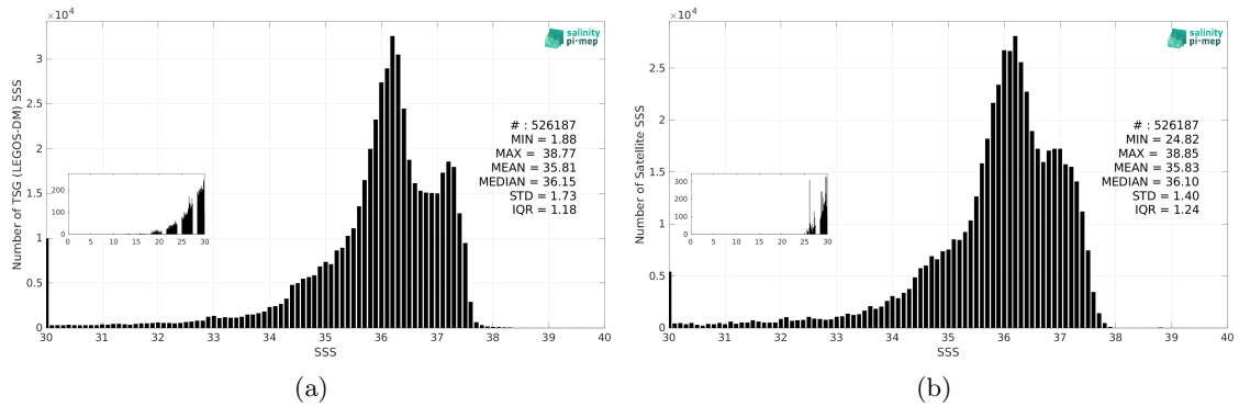
Figure 3: Histograms of SSS from TSG (LEGOS-DM) (a) and SMOS SSS L3 v335 - Monthly - 25 km (CATDS-CPDC) (b) considering all match-up pairs per bins of 0.1 over the Tropical Atlantic Ocean Pi-MEP region and for the full satellite product period.
