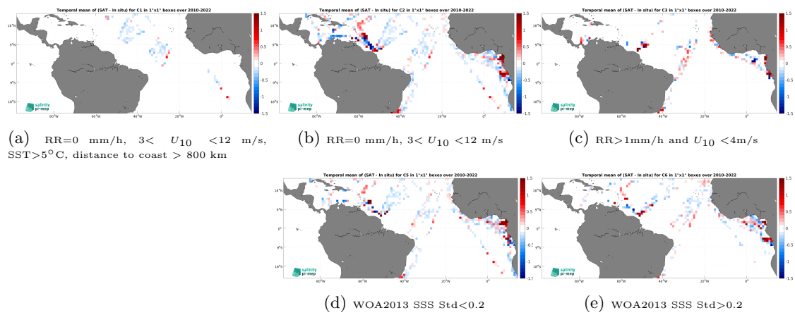
Figure 14: Temporal mean gridded over spatial boxes of size 1^\circ \times 1^\circ of \Delta SSS (SMOS SSS L3 v335 - Monthly - 25 km (CATDS-CPDC) - TSG (LEGOS-DM)) for 5 different subdatasets corresponding to:RR=0 mm/h, 3 < U_{10} < 12 m/s, SST >5^\circ\text{C} , distance to coast > 800 km (a), RR=0 mm/h, 3 < U_{10} < 12 m/s (b), RR >1 mm/h and U_{10} < 4 m/s (c), WOA2013 SSS Std <0.2 (d), WOA2013 SSS Std >0.2 (e).
