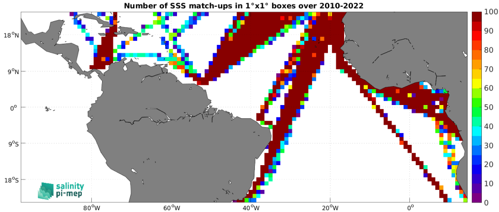
Figure 5: Number of SSS match-ups between TSG (LEGOS-DM) SSS and the SMOS SSS L3 v335 - Monthly - 25 km (CATDS-CPDC) SSS product for the Tropical Atlantic Ocean Pi-MEP region over 1^\circ \times 1^\circ boxes and for the full satellite product period.
