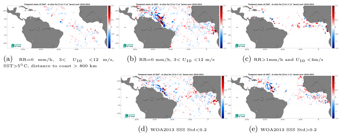
Figure 14: Temporal mean gridded over spatial boxes of size 1^\circ \times 1^\circ of \Delta\text{SSS} (SMOS SSS L3 v335 - Monthly - 25 km (CATDS-CPDC) - TSG (GOSUD-Research-vessel)) for 5 different subdatasets corresponding to:RR=0 mm/h, 3 < U_{10} < 12 m/s, SST >5^\circ\text{C} , distance to coast > 800 km (a), RR=0 mm/h, 3 < U_{10} < 12 m/s (b), RR >1 mm/h and U_{10} < 4 m/s (c), WOA2013 SSS Std <0.2 (d), WOA2013 SSS Std >0.2 (e).
