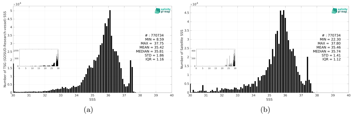
Figure 3: Histograms of SSS from TSG (GOSUD-Research-vessel) (a) and SMOS SSS L3 v335 - Monthly - 25 km (CATDS-CPDC) (b) considering all match-up pairs per bins of 0.1 over the Tropical Atlantic Ocean Pi-MEP region and for the full satellite product period.
