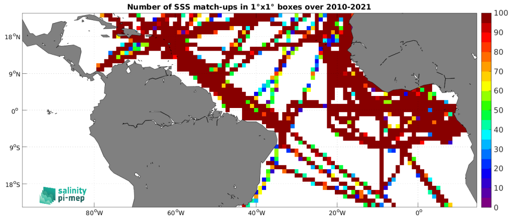
Figure 5: Number of SSS match-ups between TSG (GOSUD-Research-vessel) SSS and the SMOS SSS L3 v335 - Monthly - 25 km (CATDS-CPDC) SSS product for the Tropical Atlantic Ocean Pi-MEP region over 1^\circ \times 1^\circ boxes and for the full satellite product period.
