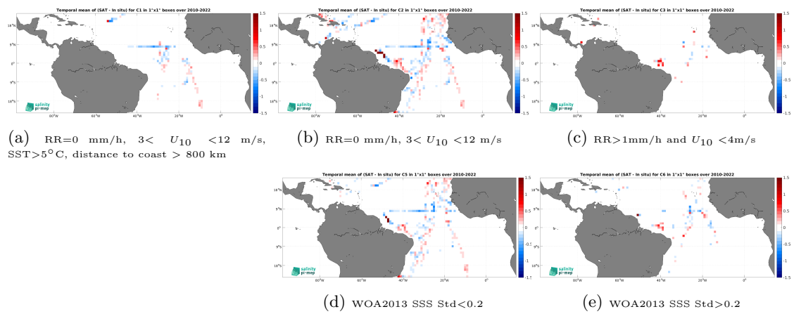
Figure 14: Temporal mean gridded over spatial boxes of size 1^\circ \times 1^\circ of \Delta SSS (SMOS SSS L3 v335 - Monthly - 25 km (CATDS-CPDC) - TSG (CSIC-UTM)) for 5 different subdatasets corresponding to:RR=0 mm/h, 3 < U_{10} < 12 m/s, SST >5^\circ\text{C} , distance to coast > 800 km (a), RR=0 mm/h, 3 < U_{10} < 12 m/s (b), RR >1 mm/h and U_{10} < 4 m/s (c), WOA2013 SSS Std <0.2 (d), WOA2013 SSS Std >0.2 (e).
