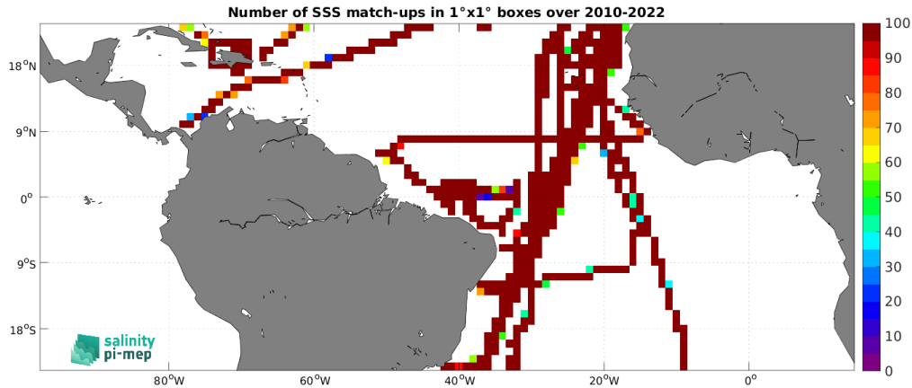
Figure 4: Number of SSS match-ups between TSG (CSIC-UTM) SSS and the SMOS SSS L3 v335 - Monthly - 25 km (CATDS-CPDC) SSS product for the Tropical Atlantic Ocean Pi-MEP region over 1^\circ \times 1^\circ boxes and for the full satellite product period.
