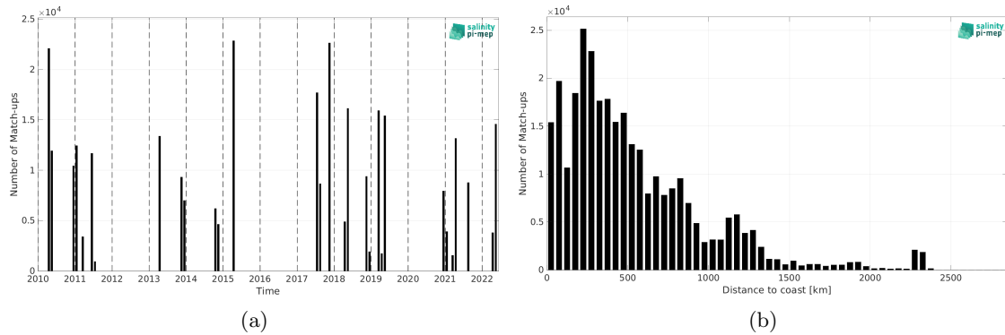
Figure 1: Number of match-ups between TSG (CSIC-UTM) and SMOS SSS L3 v335 - Monthly - 25 km (CATDS-CPDC) SSS as a function of time (a) and as function of the distance to coast (b) over the Tropical Atlantic Ocean Pi-MEP region and for the full satellite product period.
