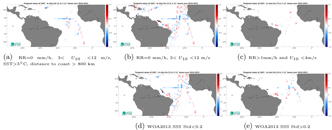
Figure 12: Temporal mean gridded over spatial boxes of size 1^\circ \times 1^\circ of \Delta\text{SSS} (SMOS SSS L3 v335 - Monthly - 25 km (CATDS-CPDC) - TSG (CSIC-UTM)) for 5 different subdatasets corresponding to:RR=0 mm/h, 3 < U_{10} < 12 m/s, SST >5^\circ\text{C} , distance to coast > 800 km (a), RR=0 mm/h, 3 < U_{10} < 12 m/s (b), RR >1 mm/h and U_{10} < 4 m/s (c), WOA2013 SSS Std <0.2 (d), WOA2013 SSS Std >0.2 (e).
