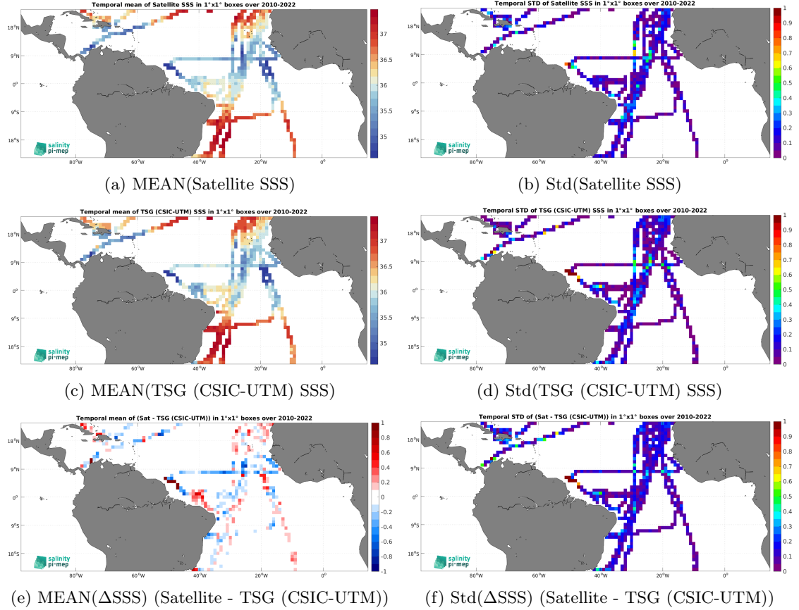
Figure 6: Temporal mean (left) and Std (right) of SSS from SMOS SSS L3 v335 - Monthly - 25 km (CATDS-CPDC) (top), TSG (CSIC-UTM) (middle), and of \Delta\text{SSS} (Satellite - TSG (CSIC-UTM)). Only match-up pairs are used to generate these maps.
