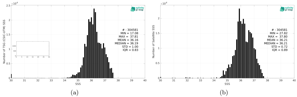
Figure 2: Histograms of SSS from TSG (CSIC-UTM) (a) and SMOS SSS L3 v335 - Monthly - 25 km (CATDS-CPDC) (b) considering all match-up pairs per bins of 0.1 over the Tropical Atlantic Ocean Pi-MEP region and for the full satellite product period.
