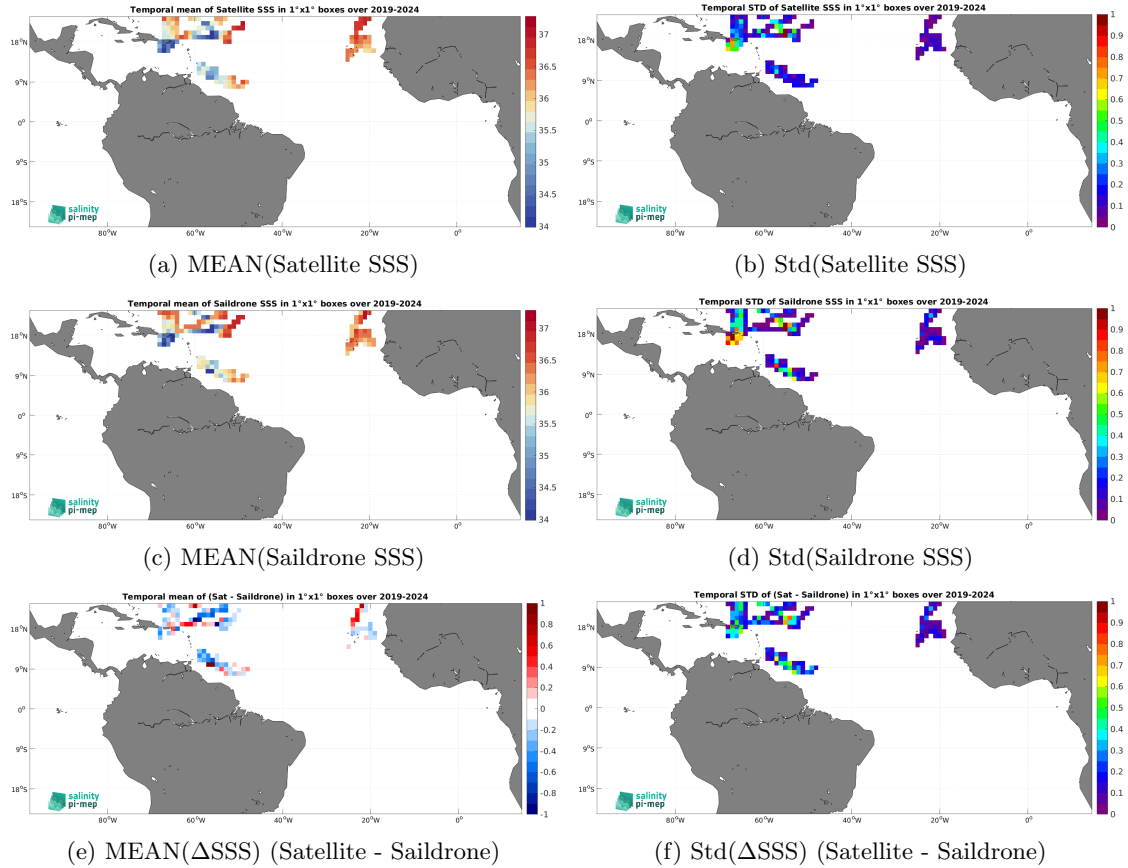
Figure 7: Temporal mean (left) and Std (right) of SSS from SMOS SSS L3 v335 - Monthly - 25 km (CATDS-CPDC) (top), Sairdron (middle), and of \Delta SSS (Satellite - Sairdron). Only match-up pairs are used to generate these maps.
