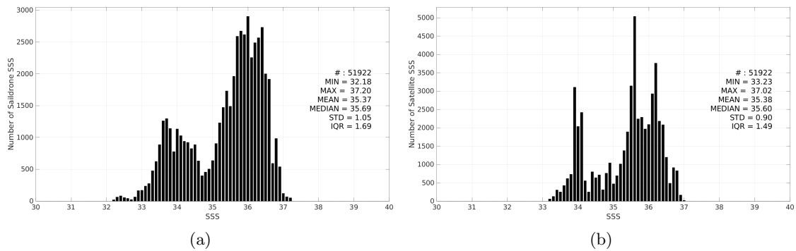
Figure 3: Histograms of SSS from Saildrone (a) and SMOS SSS L3 v335 - Monthly - 25 km (CATDS-CPDC) (b) considering all match-up pairs per bins of 0.1 over the Tropical Atlantic Ocean Pi-MEP region and for the full satellite product period.
