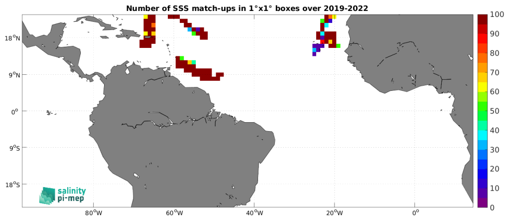
Figure 5: Number of SSS match-ups between Saildrone SSS and the SMOS SSS L3 v335 - Monthly - 25 km (CATDS-CPDC) SSS product for the Tropical Atlantic Ocean Pi-MEP region over 1^\circ \times 1^\circ boxes and for the full satellite product period.
