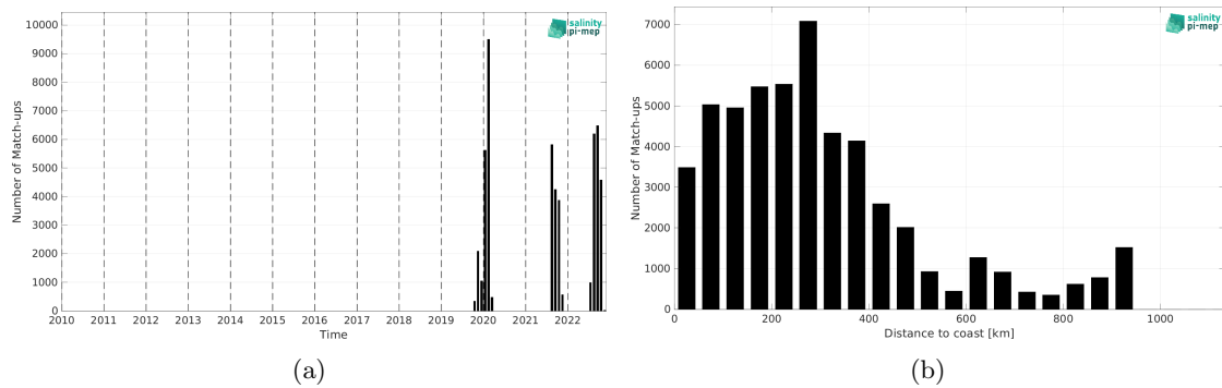
Figure 2: Number of match-ups between Saildrone and SMOS SSS L3 v335 - Monthly - 25 km (CATDS-CPDC) SSS as a function of time (a) and as function of the distance to coast (b) over the Tropical Atlantic Ocean Pi-MEP region and for the full satellite product period.
