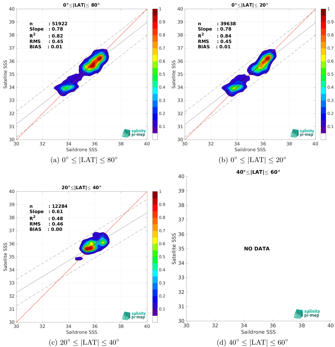
Figure 10: Contour maps of the concentration of SMOS SSS L3 v335 - Monthly - 25 km (CATDS-CPDC) SSS (y-axis) versus Saildrone SSS (x-axis) at match-up pairs for different latitude bands. For each plot, the red line shows x=y . The black thin and dashed lines indicate a linear fit through the data cloud and the \pm 95\% confidence levels, respectively. The number match-up pairs n , the slope and R^2 coefficient of the linear fit, the root mean square (RMS) and the mean bias between satellite and in situ data are indicated for each latitude band in each plots.
