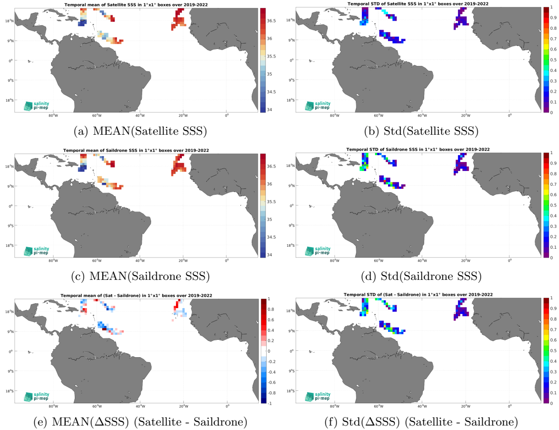
Figure 7: Temporal mean (left) and Std (right) of SSS from SMOS SSS L3 v335 - Monthly - 25 km (CATDS-CPDC) (top), Sairdron (middle), and of \Delta\text{SSS} (Satellite - Sairdron). Only match-up pairs are used to generate these maps.
