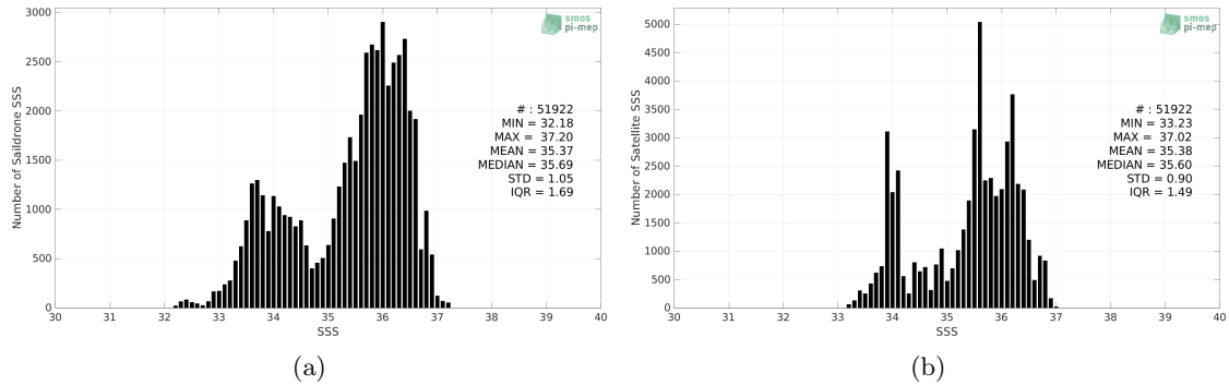
Figure 2: Histograms of SSS from Sairdrone (a) and SMOS SSS L3 v335 - Monthly - 25 km (CATDS-CPDC) (b) considering all match-up pairs per bins of 0.1 over the Tropical Atlantic Ocean Pi-MEP region and for the full satellite product period.
