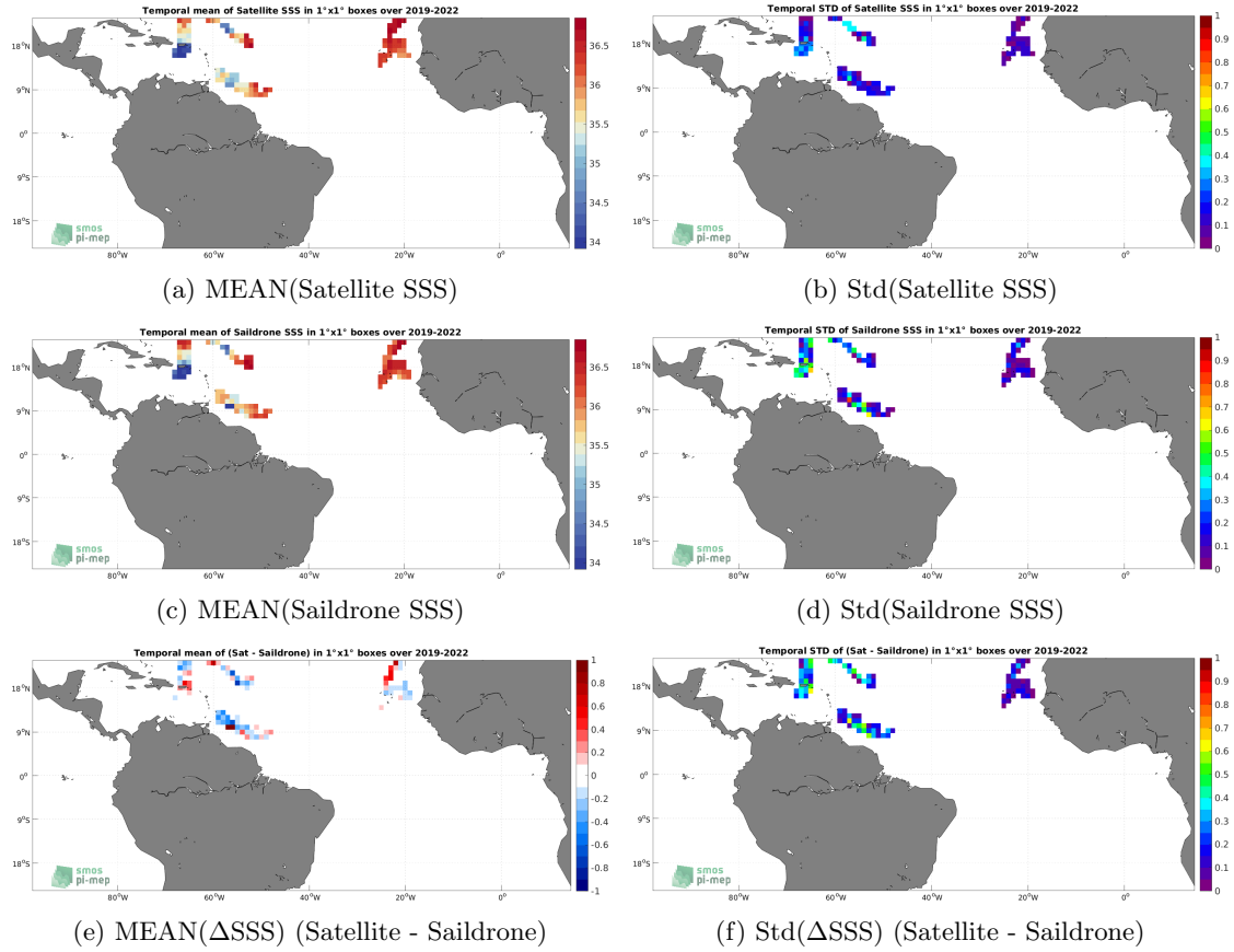
Figure 6: Temporal mean (left) and Std (right) of SSS from SMOS SSS L3 v335 - Monthly - 25 km (CATDS-CPDC) (top), Sairdrone (middle), and of \Delta SSS (Satellite - Sairdrone). Only match-up pairs are used to generate these maps.
