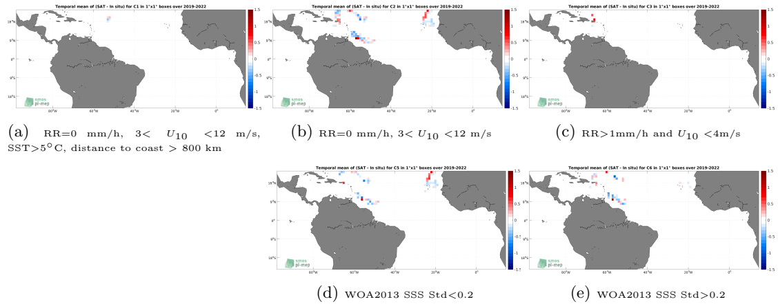
Figure 12: Temporal mean gridded over spatial boxes of size 1^\circ \times 1^\circ of \Delta SSS (SMOS SSS L3 v335 - Monthly - 25 km (CATDS-CPDC) - Sairdrone) for 5 different subdatasets corresponding to:RR=0 mm/h, 3 < U_{10} < 12 m/s, SST >5^\circ\text{C} , distance to coast > 800 km (a), RR=0 mm/h, 3 < U_{10} < 12 m/s (b), RR >1 mm/h and U_{10} < 4 m/s (c), WOA2013 SSS Std <0.2 (d), WOA2013 SSS Std >0.2 (e).
