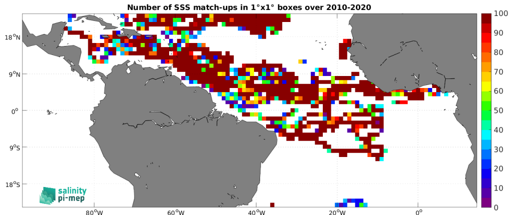
Figure 4: Number of SSS match-ups between Surface drifters SSS and the SMOS SSS L3 v335 - Monthly - 25 km (CATDS-CPDC) SSS product for the Tropical Atlantic Ocean Pi-MEP region over 1^\circ \times 1^\circ boxes and for the full satellite product period.
