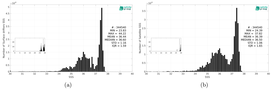
Figure 3: Histograms of SSS from Surface drifters (a) and SMOS SSS L3 v335 - Monthly - 25 km (CATDS-CPDC) (b) considering all match-up pairs per bins of 0.1 over the Tropical Atlantic Ocean Pi-MEP region and for the full satellite product period.
